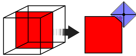
Figure 3: (Left) The large red plane is the current kd split plane. (Right) the split plane is isolated, the beam is in blue, and our viewpoint is down the axis of the beam pyramid. In this case, the beam’s corner rays only want to traverse the far cell, but, clearly, we also need to visit the near cell.
