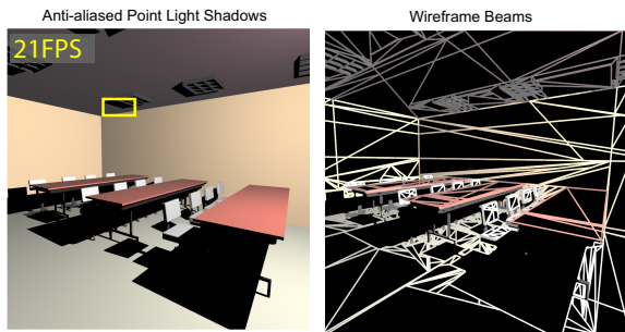
Figure 9: Real-time antialiased point light shadows. (Left) This image was rendered at 21 frames per second at 1024x1024 resolution with 6\times antialiasing inside the 2 million triangle soda hall model. (Right) The wireframe beams which generated the top-left image: all geometry and shadows are cut out exactly providing for high-quality antialiasing (Fig. 10).
