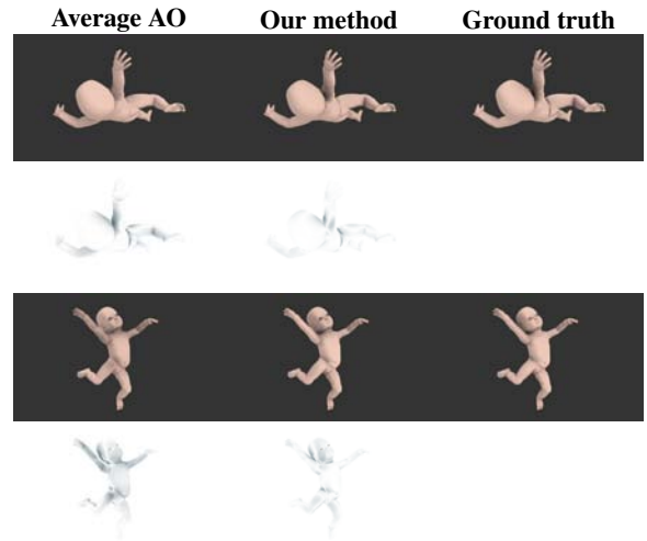
Figure 4: Static average ambient occlusion (Left) and our method (Middle) compared against the ground truth (Right). The ground truth was obtained by tracing 1000 quasi-random rays per vertex. The second and fourth rows show the difference images against the ground truth.
