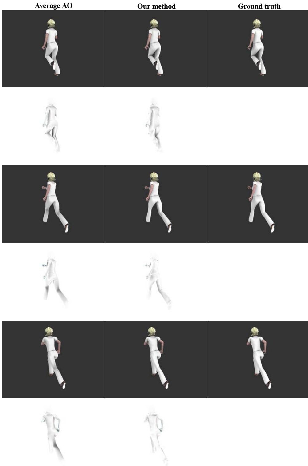
Figure 5: Static average ambient occlusion ( Left ) and our method ( Middle ) compared against the ground truth ( Right ). The ground truth was obtained by tracing 1000 quasi-random rays per vertex. The second, fourth, and sixth rows show the difference images against the ground truth.
