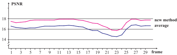
Figure 3: Peak signal-to-noise ratio (PSNR) of ambient occlusion during 30 frames when Jessi is running. The error is evaluated against a ray traced reference solution. Higher PSNR indicates less error. Clearly, the new method gives consistently better approximation of ambient occlusion.
