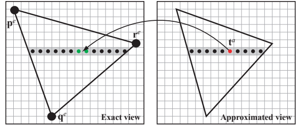
Figure 5: Illustration of how a fragment (red circle) with perspective-correct barycentric coordinates t^a , in an approximated view, can be mapped onto a screen-space position in the exact view. The color of two nearby fragments in the exact view are interpolated to compute the color of the fragment in the approximated view.
