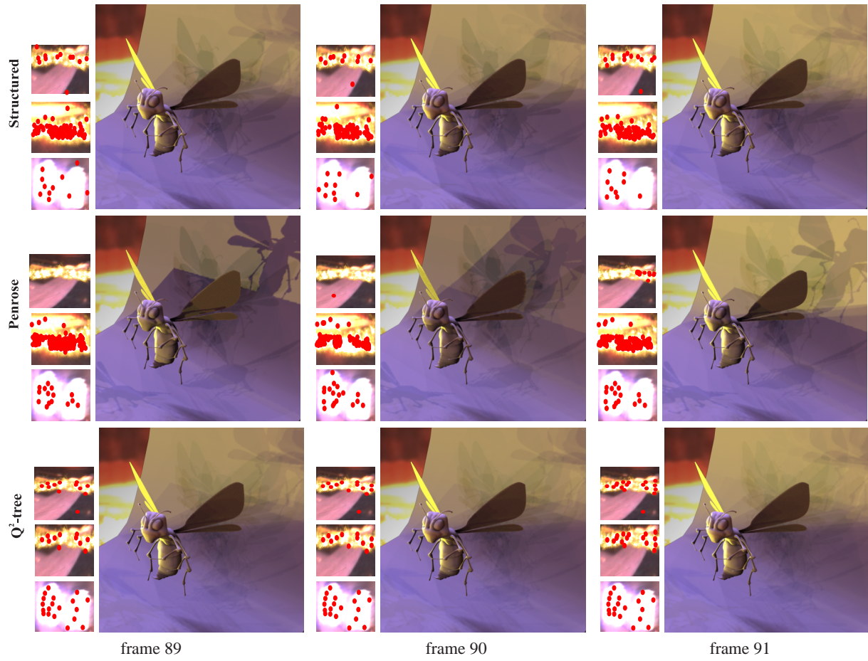
Color Figure 10: Comparison of structured, Penrose and Q^2 -tree sampling methods in terms of temporal consistency.
