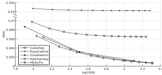
Figure 4: Discrepancy of various sampling patterns. In general, the discrepancy decreases as the number of samples, N , increases.
