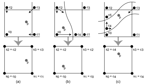
Figure 6: Bilinear interpolation using neighboring reachable samples. Texel representative samples are in the lower left corners of the texels. If all 4 samples are not available, existing samples are used instead. (a) Standard texture mapping. (b) The right side samples are blocked, so the ones on the left are copied, preserving the gradient. (c) Only the upper right sample can be reached.
