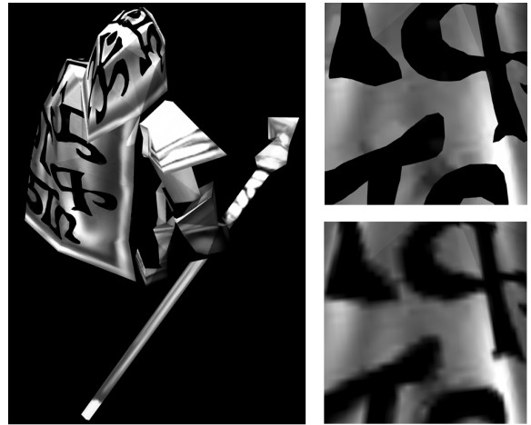
Figure 11: Comparisons of wizard model. Left: Antialiased rendering of model using an FBT skin. Right: zoomed-in comparison (Top: FBT; Bottom: original raster skin). Artwork from Warcraft III®: Reign of Chaos™ provided courtesy of Blizzard Entertainment.
