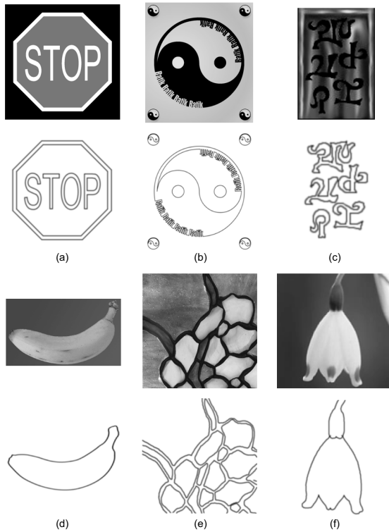
Figure 7: Example inputs and their corresponding features. (a) and (b) are SVGs; (c), (e), and (f) are raster images annotated by hand using line segments; (d) is a raster image annotated by Potrace using splines.
