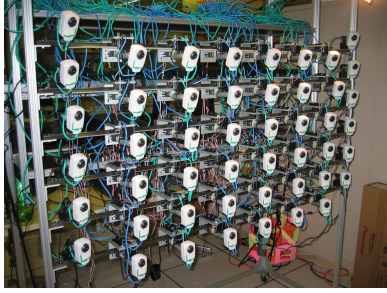
Figure 1: Our self-reconfigurable camera array system with 48 cameras.
