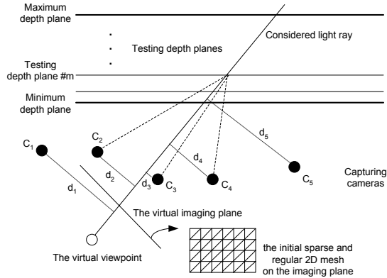
Figure 7: Locate the neighboring images for interpolation and depth reconstruction through plane sweeping.
