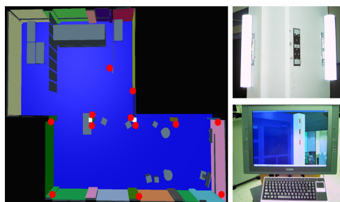
Figure 3: 3D model of the laboratory with targets marked as red circles (left). Flexible target attachment at pillars (right top) and a live image from the evaluation (right bottom).
