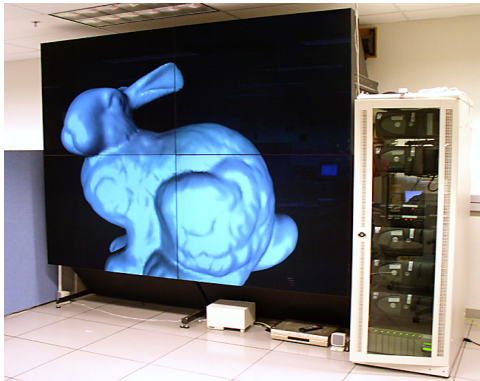
Figure 2: Setup of our test bed showing the two-by-two tiled display wall and the rendering cluster.
