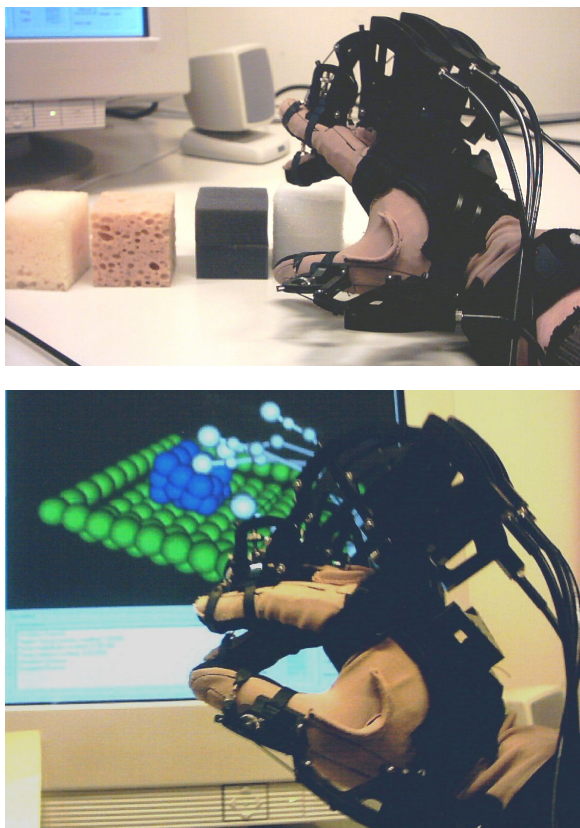
Figure 7: Testing reaction force of different objects
