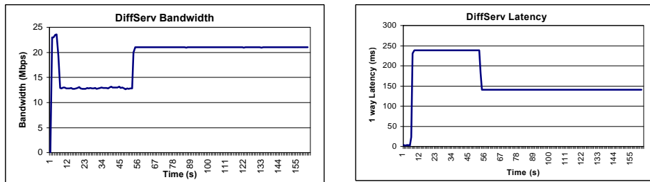
Fig. 3. Results showing that DiffServ, while being able to make bandwidth guarantees, may not always provide latency guarantees.
