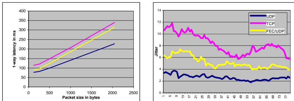
Fig. 4. The graph on the left shows the transmission of 100 packets under TCP, UDP, FEC/UDP. The FEC scheme derives its greatest benefit when packet sizes are small as larger packet sizes incur additional buffer processing time. The graph on the right shows that FEC also introduces jitter in the data stream. Jitter is computed by first calculating the short-term latency over every 20 data points and then computing the average deviation of the instantaneous latency as compared to the short-term latency.
