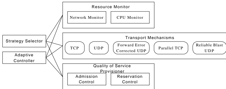
Fig. 1. Components of an Adaptive Networking System
