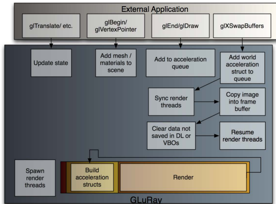
Figure 2: Parallel architecture of GLuRay.
