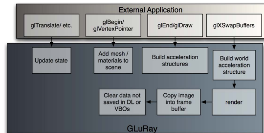
Figure 1: Sequential architecture of GluRay.
