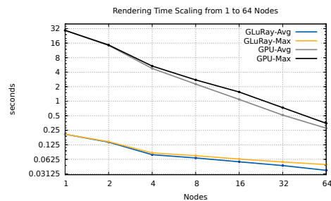
Figure 10: Rendering times for the RMO dataset in ParaView using the Longhorn visualization cluster. "Avg" denotes the averaged render times across every node while "Max" designates the maximum render time across all nodes.
