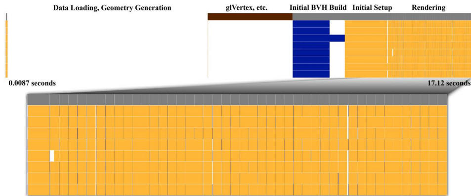
Figure 9: Gantt charts showing a rendering of a wavelet dataset with 8 million triangles. An overall view of setup time, geometry transfer, acceleration builds and rendering is shown in the top runs while a closeup of the rendering is shown in the bottom. The gold color displays the efficiency of the asynchronous renderer while the blue displays the cost of BVH builds in relation to data loading and geometry specification through OpenGL shown in brown.
