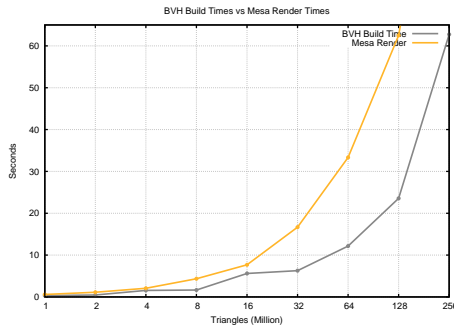
Figure 8: BVH build times for the wavelet dataset compared to Mesa rendering time for a single frame.
