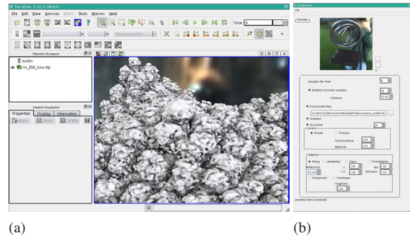
Figure 3: GLuRay running within ParaView (a) and an external GUI (b).
