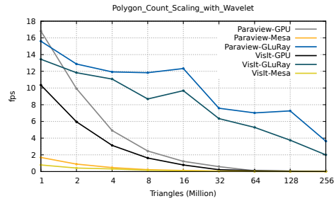
Figure 7: Performance timings for increasing triangle counts for a wavelet dataset as seen in Figure 6(c).
