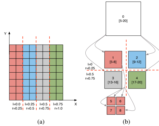
Figure 4: Sort-last database decomposition of terrain for four nodes using (a) linear block and (b) quadtree enumeration.
