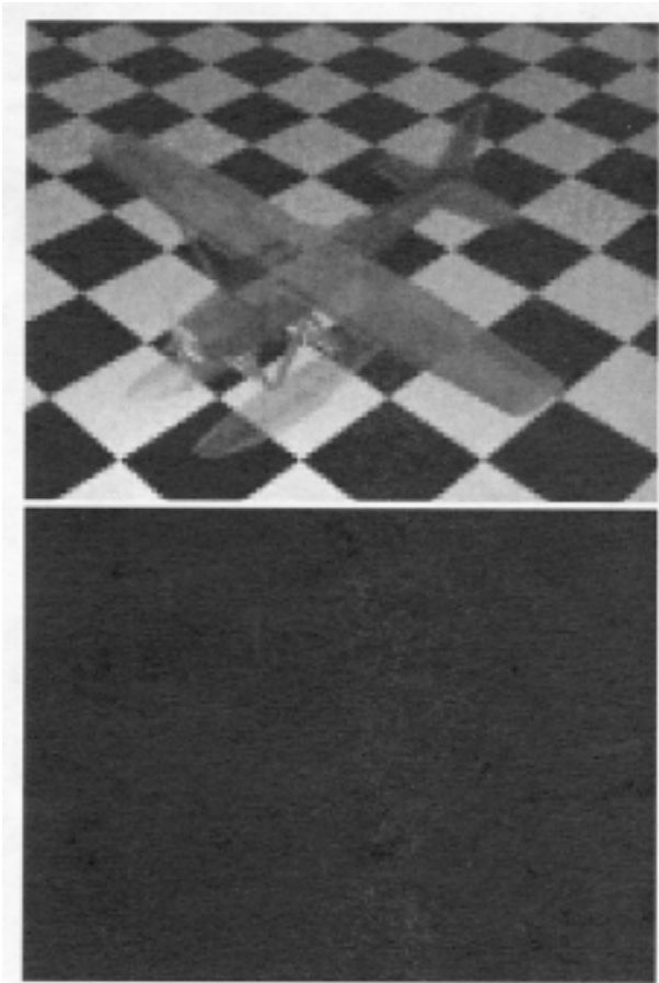
Figure 11: The transparent Cessna seaplane using Z^3 with 16 samples on a 16 \times 16 grid and storage for 4 fragments per pixel. The lower figure gives the per-pixel difference from a 16X sparse supersampled reference image with an unbounded number of fragments. (Also in the color section.)
