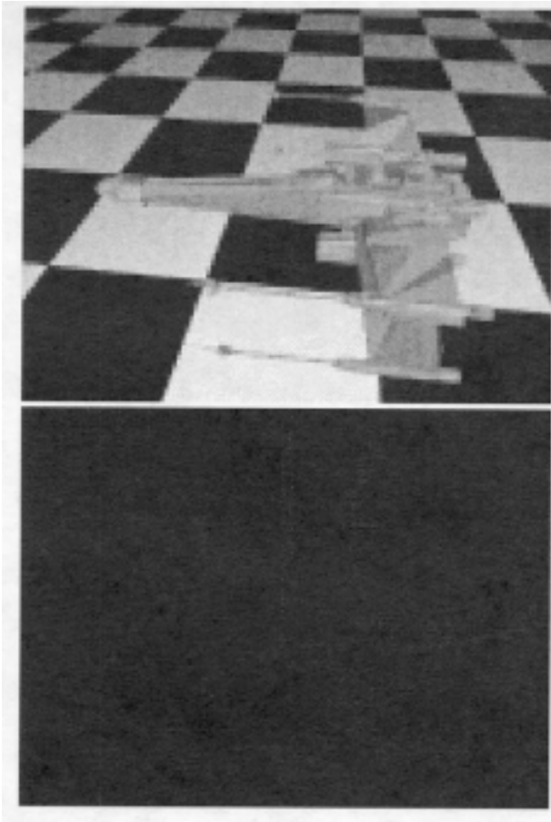
Figure 9: The x-wing fighter using Z^3 with 16 samples on a 16 \times 16 grid and storage for 3 fragments. The lower figure gives the per-pixel difference from a 16X sparse supersampled reference image. (Also in the color section.)
