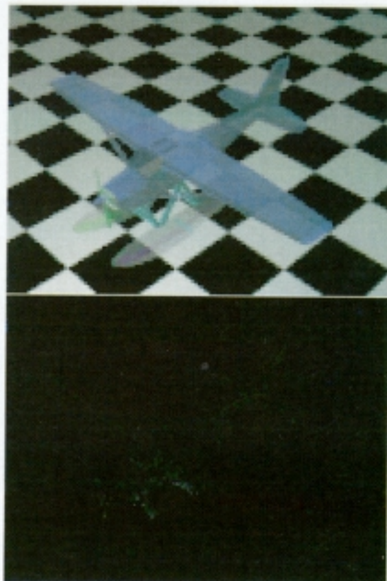
Figure 11: The transparent Cessna seaplane with 16 samples on a 16 \times 16 grid and storage for 4 fragments per pixel. The lower figure gives the per-pixel difference from a 16X sparse supersampled reference image with an unbounded number of fragments.
