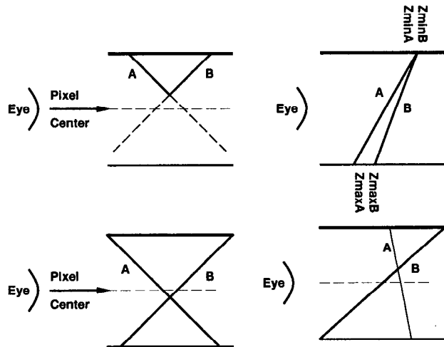
Figure 1: Difficult cases for non-complete Z information.
