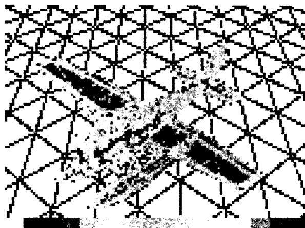
Figure 3: The color represents the maximum number of fragments that are visible in each pixel of one frame of the transparent Cessna test case when using 16 samples per pixel. The color code at the bottom shows the colors representing 1 (white) to 16 or more (red). Some pixels have as many as 30 fragments. (Also in the color section.)
