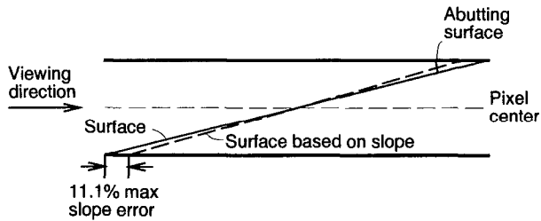
Figure 5: Implications of inaccurate slopes.
