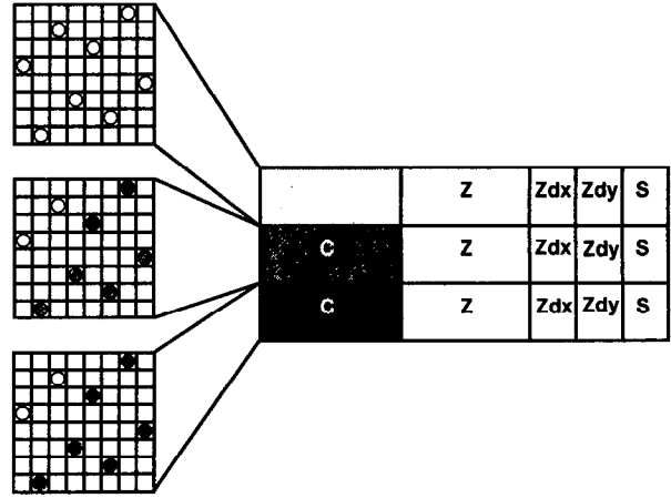
Figure 4: The Z^3 data structure, which is used to provide antialiasing and order-independent transparency. In this example each of the three fragments has an associated coverage mask, which contains 8 samples on an 8 \times 8 grid. Implementations vary in the number of sample points and fragments. This data structure is used in addition to conventional storage of per-pixel final color and Z information in front and back buffers.
