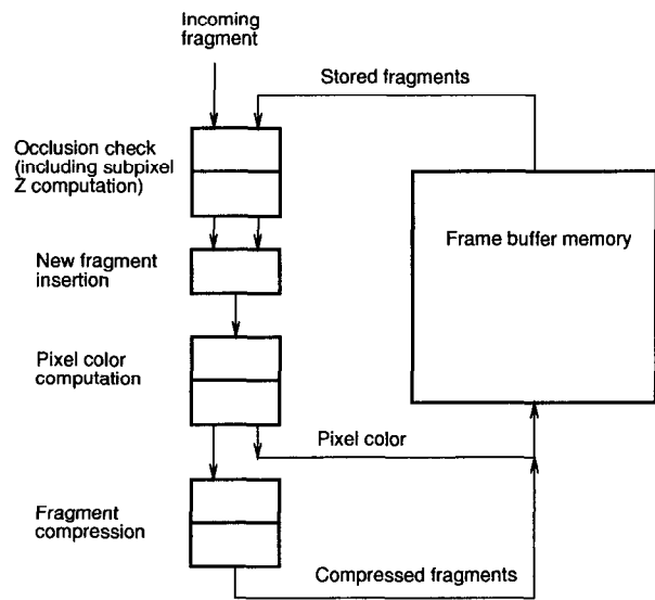
Figure 6: The Z^3 fragment processing pipeline.
