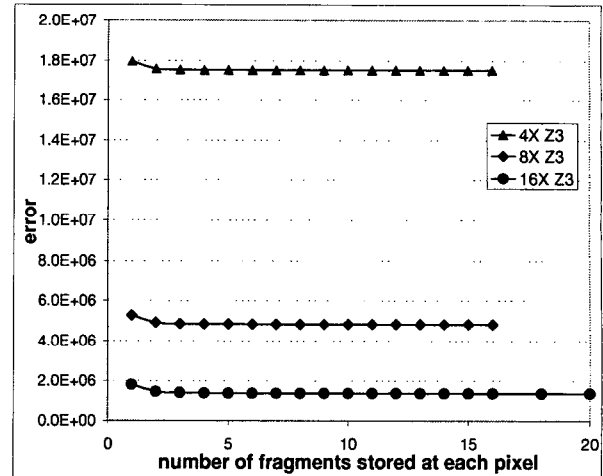
Figure 10: The errors introduced by 4 \times , 8 \times , and 16 \times Z^3 with various numbers of fragments for the transparent Cessna test case. The reference image is rendered by 32 \times sparse supersampling with an unbounded number of fragments.
