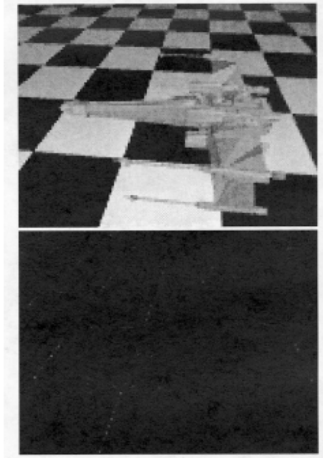
Figure 8: The x-wing fighter with traditional 4 \times sparse supersampling (using 4 samples on a 4 \times 4 grid). The lower figure gives the per-pixel difference from a 16 \times sparse supersampled reference image.
