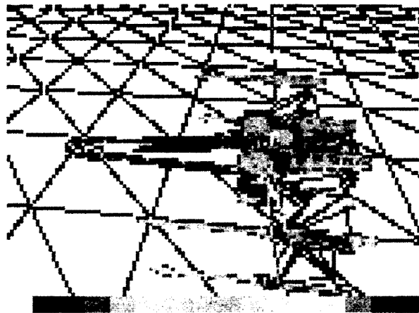
Figure 2: The color represents the maximum number of fragments that are visible in each pixel of one frame of the x-wing test case when using 16 samples per pixel. The color code at the bottom shows the colors representing 1 (white) to 16 (red). (Also in the color section.)
