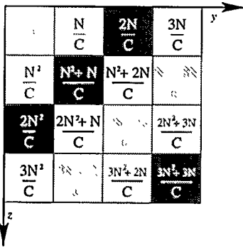
Figure 3: Memory location assignments of YZ face
