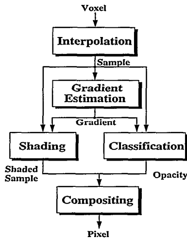
Figure 1: Rendering pipeline
