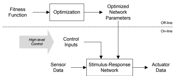
Figure 11: Neural-network-based motion control with off-line optimization.
