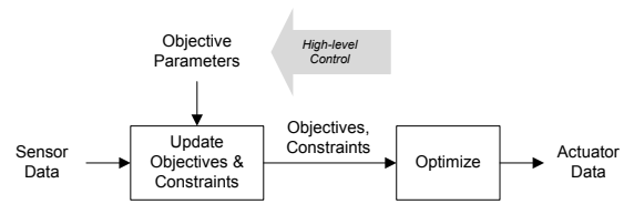
Figure 13: Optimization-based motion control.
