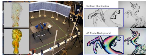
Figure 9: Schlieren imaging for tomographic gas reconstruction (left) and capture of refractive events using light field probes (right). (Figures reproduced from [AIH*08] and [WRH11].)
