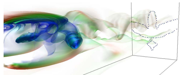
Figure 2: A set of streamsurfaces on a simulation of flow behind a cuboid [CSB105]. Transparency is mapped to surface curvature. The seeding curves can be seen on the far plane of the domain.
