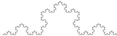
Figure 9: The Koch Curve Level 5
