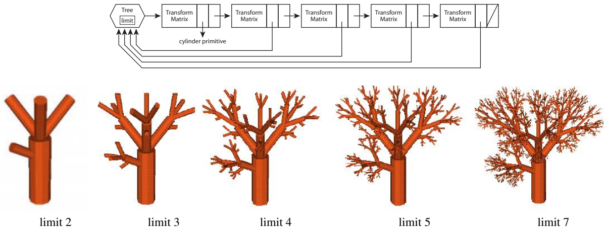
Figure 4: Top: a multiply instanced DCG definition to draw a cylinder tree. Bottom: output from this with different limits.
