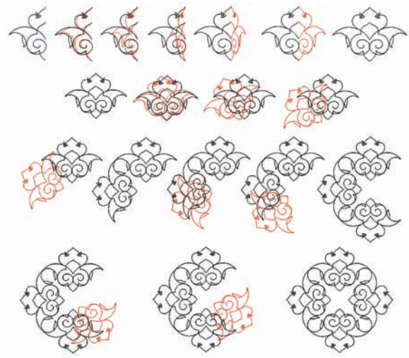
Figure 7: Visualizing the symmetry in a simple pattern.
