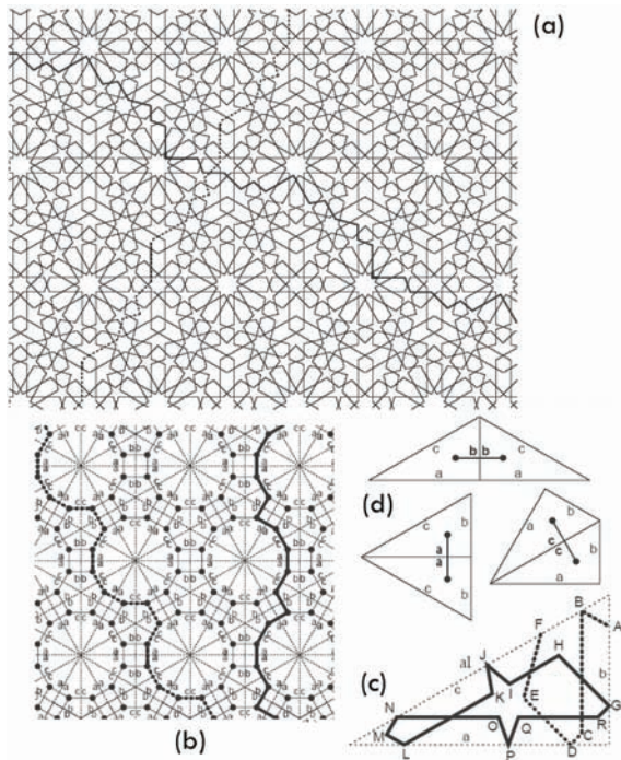
Figure 6: A schematic representation for the symmetric pattern (a) [Ost98]. (b) shows the motif, (c) its Cayley diagram, and (d) three possible interrelations between motifs. Although all elements have been carefully labeled, it is hard to conceive how pattern (a) is built from (c).
