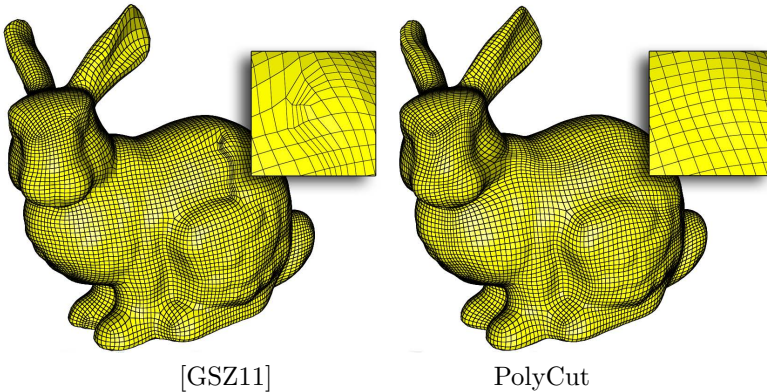
Figure 2.15: Hex-meshing is a typical application for PolyCube mappings. Here both a quality (see table) and a visual (see bunnies on the bottom line) comparison with Gregson et al is provided. In the table, from left to right: minimum and average Scaled Jacobian for the two methods, improvement factor for Minimum Scaled Jacobian. PolyCut generates better PolyCubes that dramatically increase the worst element quality, a critical metric for analysis accuracy.
