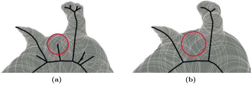
Figure 3.1: A visual comparison between MAT (left) and SAT (right). By applying uniform scaling SAT gradually ignores small-scale features as their maximal disks undergo a smaller growth and are included into bigger disks representing higher-scale features of the shape. The red disk, which is maximal in (a) is no longer maximal in (b) (image courtesy of [GMPW09]).
