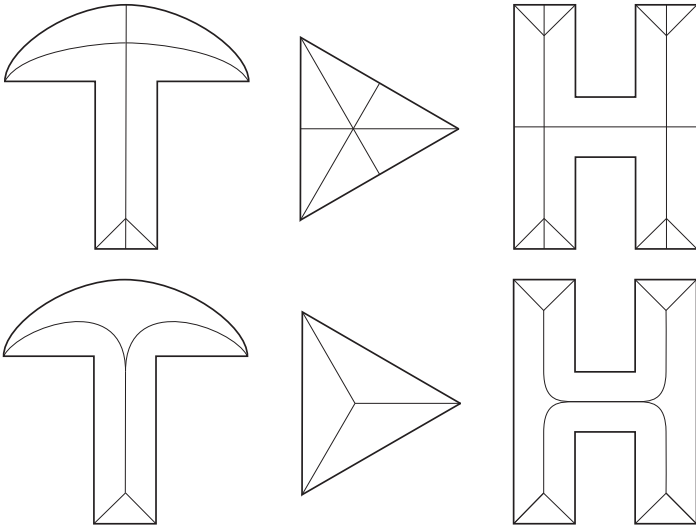
Figure 3.3: A visual comparison between SLS (top) and MAT (bottom). Strictly following the definition of symmetry set the smoothed local symmetry is able to detect more symmetry than the medial axis.
