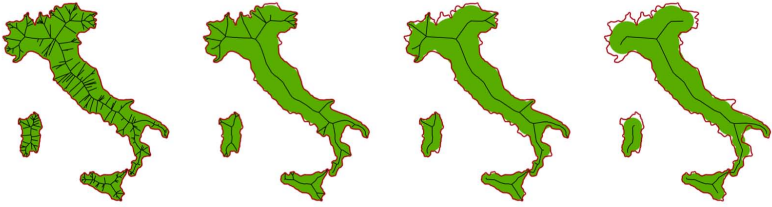
Figure 3.2: Skeletons of the map of Italy computed using SAT at growing scales (left to right). The red line denotes the boundary of the original domain. Green is the area reconstructed from the scale axis transform. Greater scales progressively ignore small features and catch only the essential parts of the shape (image courtesy of [GMPW09]).
