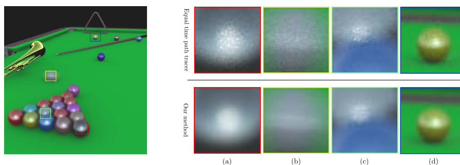
Figure 5.10 – We compare insets of the rendering of the snooker scene from our method and from a path tracer using the same amount of time. We show here that using filters allow to get a noise-less image.
