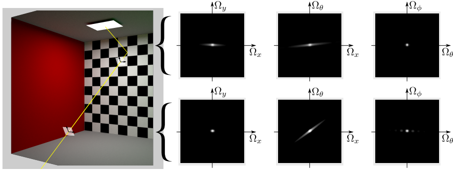
Figure 3.11 – We display slices of the Fourier amplitude. The shear effect is visible on the spatio-angular slice. Indirect effects of the shear are visible in the spatial slice as a part of the energy goes to the angular domain.
