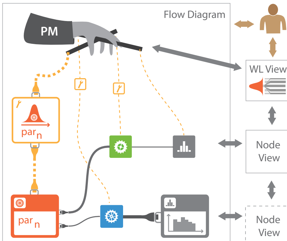
Figure 4.4 – Proposed solution: The simulation setup is presented in a data-flow diagram that is extended by a meta-flow (yellow, dashed lines) to decouple parameter control from data propagation. World Lines (WL) navigates via the puppet master (PM), a special meta-node which employs meta-communicators (yellow nodes) to control other nodes. The meta-flow highlights the control path to the red node, since in the WL view, the user studies uncertainties with respect to par_n (red). The thickness of data-flow wires (grey lines) reflects scalar values of computed results on a per-wire basis. The robustness-analyzer nodes (grey) show more detailed information.
