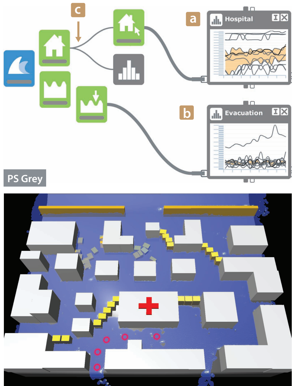
Figure 4.16 – Robustness analysis of PS Grey. The flow diagram shows detailed risk curves for (a) the damage of the hospital and (b) the water levels along the evacuation path. Neither the hospital nor the evacuation path can be considered safe. (c) There are no details about the global damage since in all cases, the damage is high. For these reasons, the barrier arrangement clearly fails with respect to all criteria.
