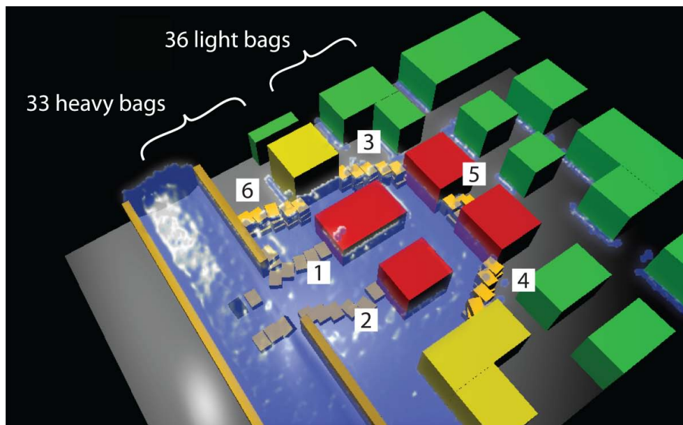
Figure 2.25 – Final solution. 70% of the buildings are protected by a multi-barrier system that consists of 6 embankments. The ordering in which the barriers are to be constructed is depicted through the numbers.
