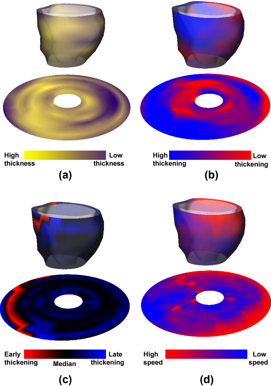
Figure 4.4. Visualization of cardiac parameters on epicardium and endocardium surfaces, and on bull's eye plots: (a) thickness; (b) thickening; (c) moment of maximum thickening; (d) speed.
