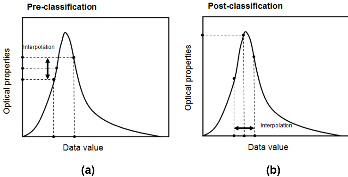
Figure 3.2. Optical property mapping for (a) pre-classification and (b) post-classification.
