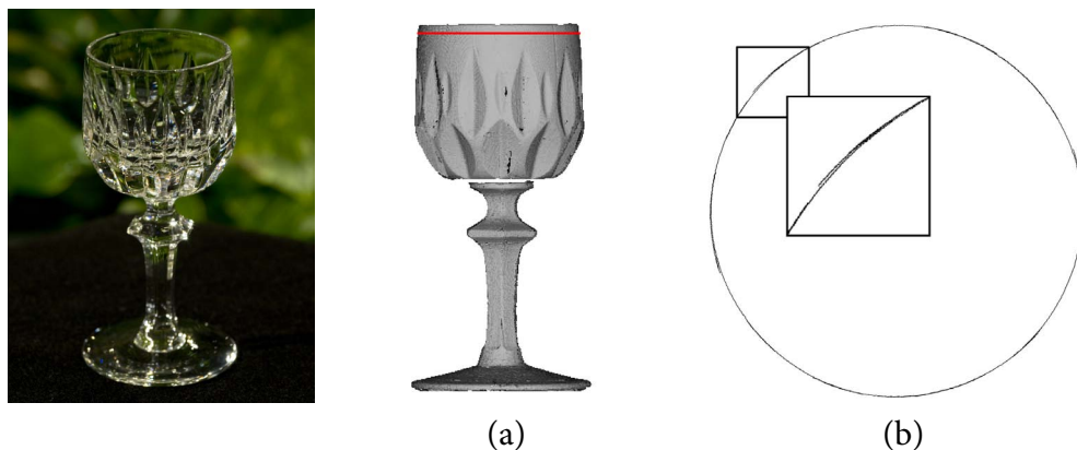
Figure 3.18: For a quantitative analysis of our first-surface scanning method, we took a cross-section of the goblet model (red line in (a)) and fitted an ellipse against it. Given 3000 sample points (b), we obtained an RMS error of 0.046 mm at an object diameter of 43.2 mm. The slight misalignment of the individual scans could probably be leveraged by geometry post-processing.
