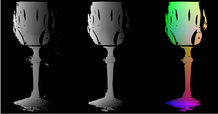
Figure 3.14: Scan maps generated from space-time stack. From left to right: depth map t(u, v) before and after segment size filtering, world coordinate map (x, y, z) . Colours are normalised for print.
