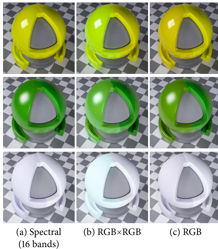
Figure 4.16: Comparison renderings using 3 different measured fluorescent materials. Full bispectral BRRDF measurements (right half of each sphere) are compared to: spectral measurements, RGBxRGB reradiation matrices, and standard RGB BRDFs.
