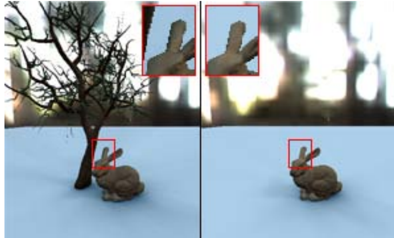
Figure 27: An object (bunny) may act as both occluder and receiver. The bunny as a receiver (left) has shadows cast on it, in contrast to the bunny (right) which act only as an occluder.
