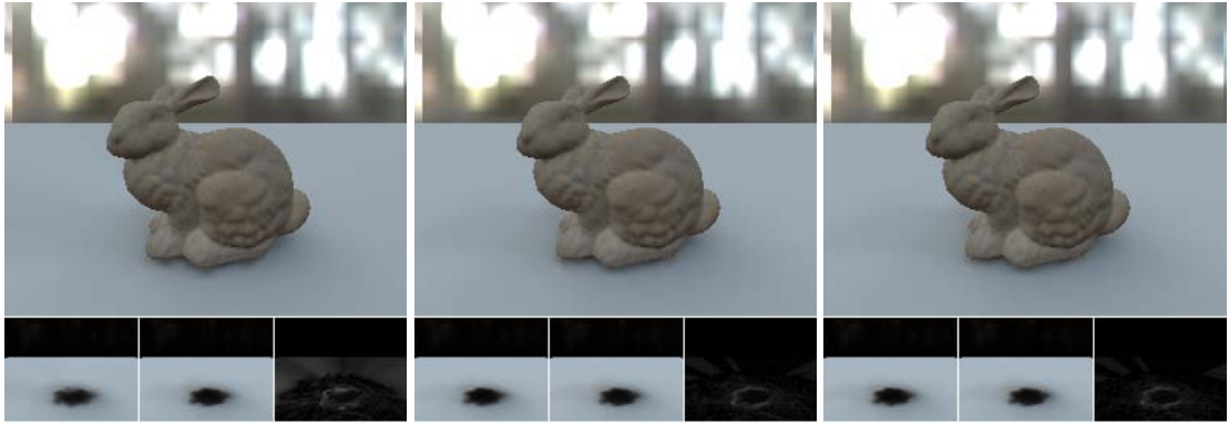
Figure 18: The bunny at different sampling rates ( \vartheta, \varphi, \varrho ): Samples = (32,17,15) (NRMSE = 0.023) (left), Samples = (64,33,30) (NRMSE = 0.008) (middle), Samples = (256,129,30) (NRMSE = 0.007) (right). The small images show the shadow only of the result of the proposed technique (left), the ground truth shadow (middle) and the difference of the two (right).
