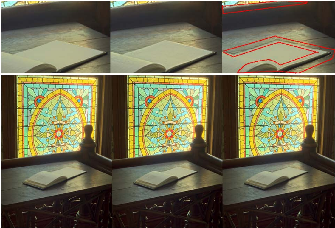
Figure 32: Tonemapped results of Desk image; close-up at the book area (top) and full resolution image (bottom). Results are given for selective tonemapping using sobel filter (left), local tonemapping (middle), selective tonemapping using saliency map (right). Artifacts in the transition areas between dark and bright regions, are strongly visible in the output obtained when saliency map is used (red marked areas).
