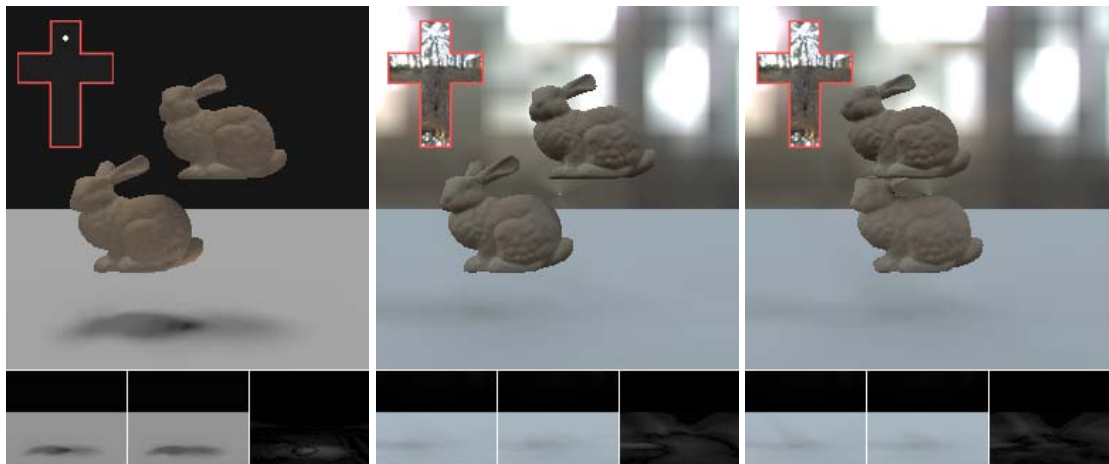
Figure 22: Illumination of multiple occluders in different parameters: 1 area light source (NRMSE = 0.019) (left), Eucalyptus grove environment map (NRMSE = 0.015) (middle), occluders in shorter distance (NRMSE = 0.013) (right).
