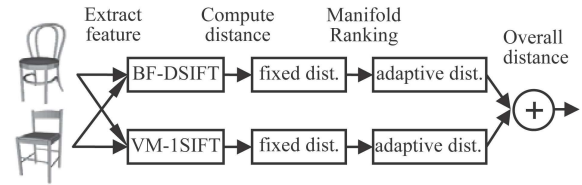
Figure 4: Two feature-adaptive distances computed using two visual features (BF-DSIFT and VM-1SIFT) are combined.
