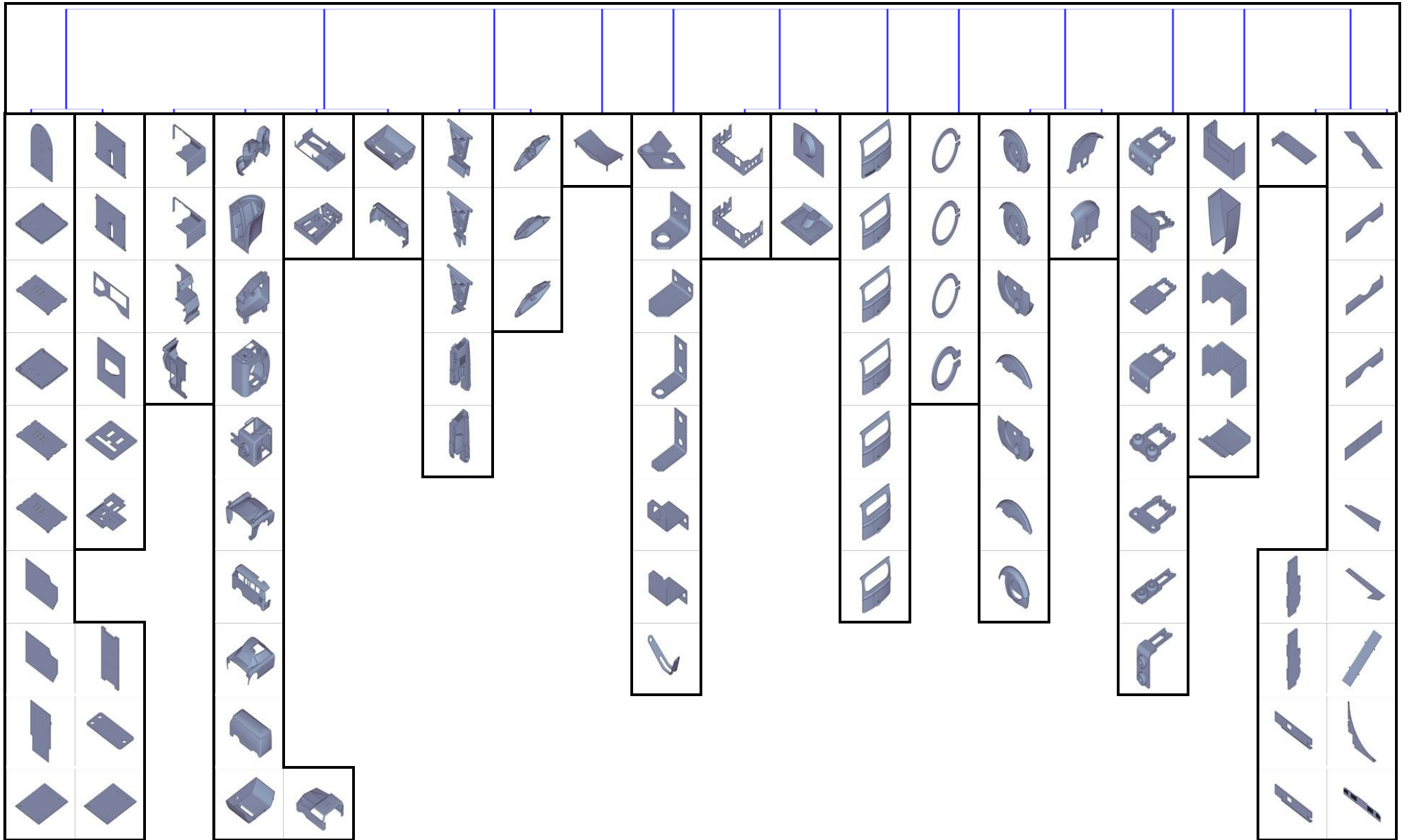
Figure A.2 Complete linkage clustering
