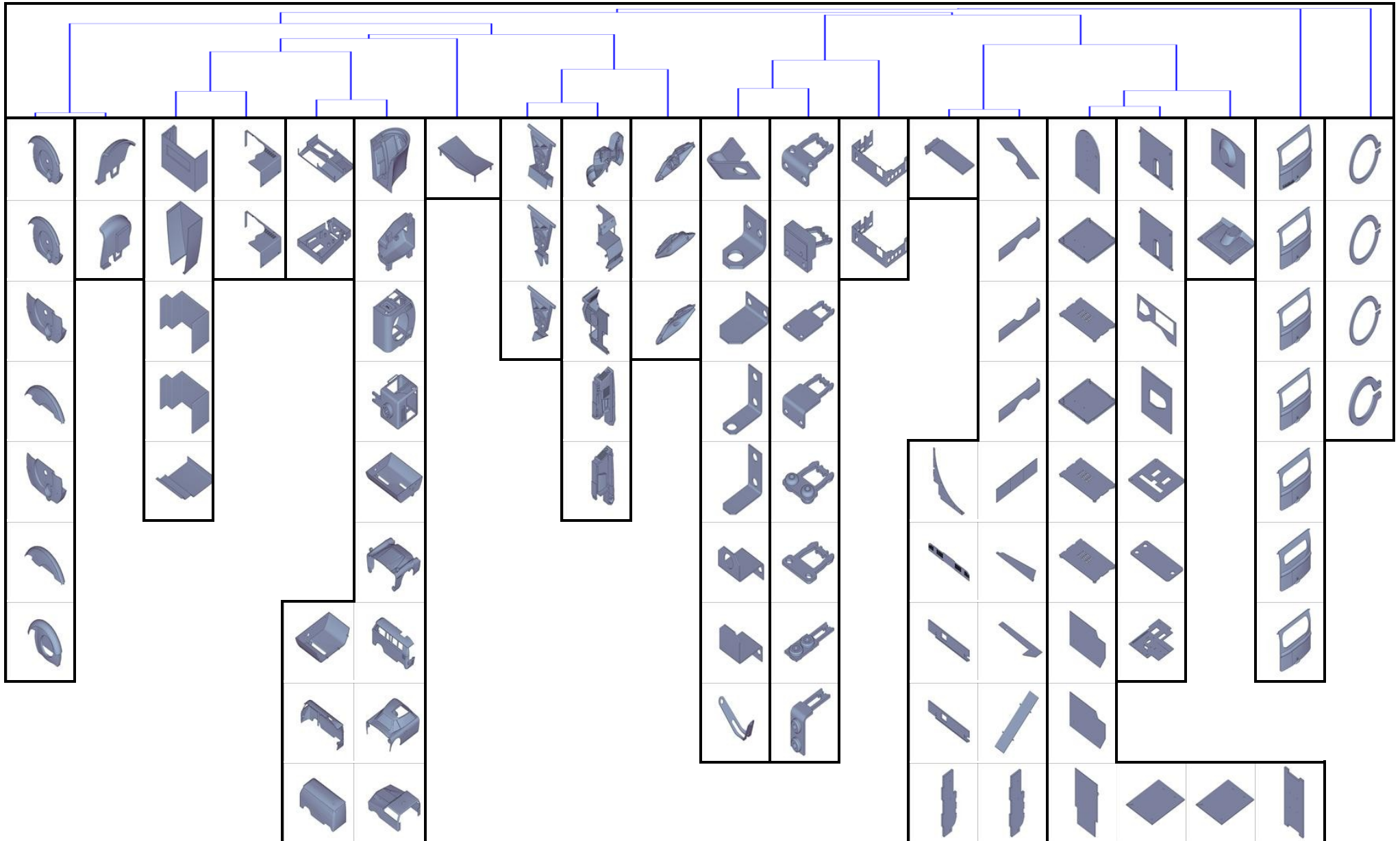
Figure A.1 Average linkage clustering
