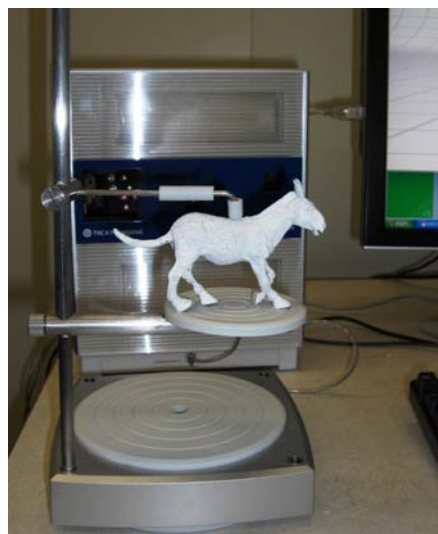
Figure 4: The setup for the acquisition of the range images.
