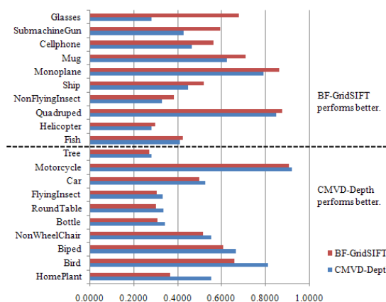
Figure 9: DCG values with respect to the query views. For the first 10 objects BF-GridSIFT method gives higher DCG values whereas for the last 10 objects CMVD-Depth method performs better.
