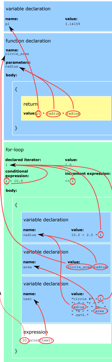
Figure 4.4: A very important data structure within a compiler is the abstract syntax tree (AST), which represents the input source code in a language-independent way. It consists of a tree structure to encode the hierarchical, nested statements (right) enriched by references to resolve symbols (visualized in red). Additional data structures – such as a table of symbols (left) – simplify the work performed by the compiler’s middleware.
