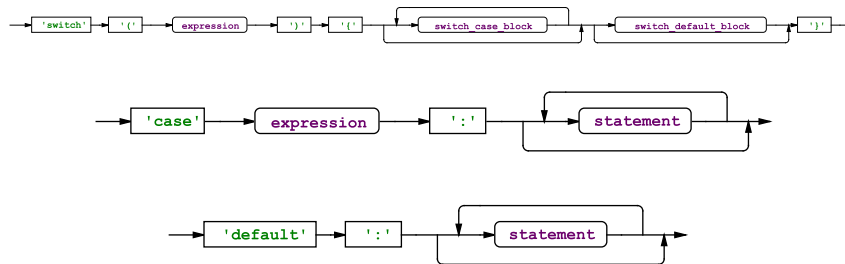
Figure A.11: A switch statement (top) consists of a selection expression, zero or more case blocks and an optional default block. The case block (middle) starts with the keyword case followed by an expression, which is compared to the selection expression, and optional statements, which are executed, if the comparison reveals equality. The optional default block (bottom) at the end of a switch statement is executed, if no case block has been executed before.
