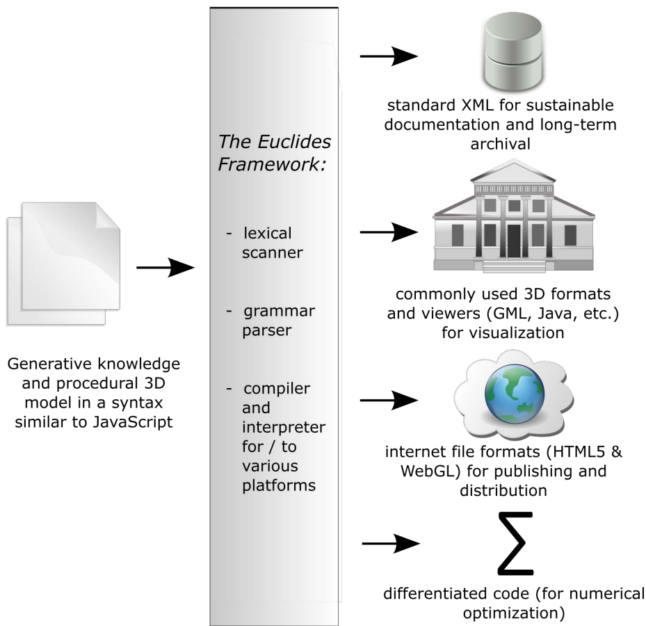
Figure 4.1: The meta modeler approach offers compiler and interpreter for many platforms, a XML target for archival, Java and GML as exemplary 3D target platforms, a HTML/WebGL target, and a target for numerical optimization.
