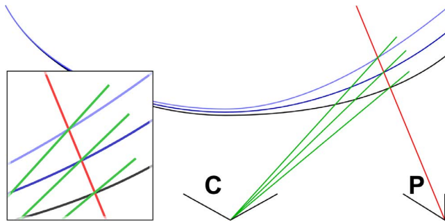
Figure 6.5: A ray from projector P (red) intersects the deforming surface on a straight line; locally, the displacement is linear with respect to the displacement of the rod, which explains the linearity observed by the camera C (green).
