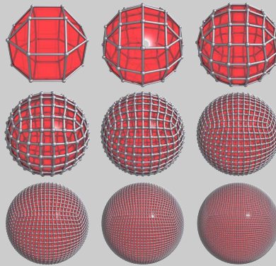
Figure 5.9: The compression scheme can represent only a limited number of normals for a fixed resolution. These configurations are visualized using 24 vertices (5 bits, top-left), and up to 7776 vertices (13 bits, bottom-right).
