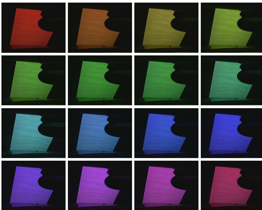
Figure 6.14: The color calibration step reduces color shifting effects caused by displays and camera. These 16 images show the captured results of fully saturated colors with varying hue spread evenly across the RGB color space.
