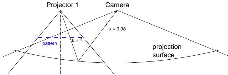
Figure 6.6: A camera acquires the checkerboard pattern that is projected on the screen. For each grid point of the pattern, the u -coordinates (in the one-dimensional example) can be measured in the camera image. These coordinates can be directly used as texture coordinates to generate an undistorted projection from the viewpoint of the camera.
