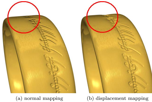
Figure 3.14: The comparison of normal mapping (a) and displacement mapping (b) reveals visual deficiencies at the silhouette as well as a lack of “depth” when using normal mapping.
