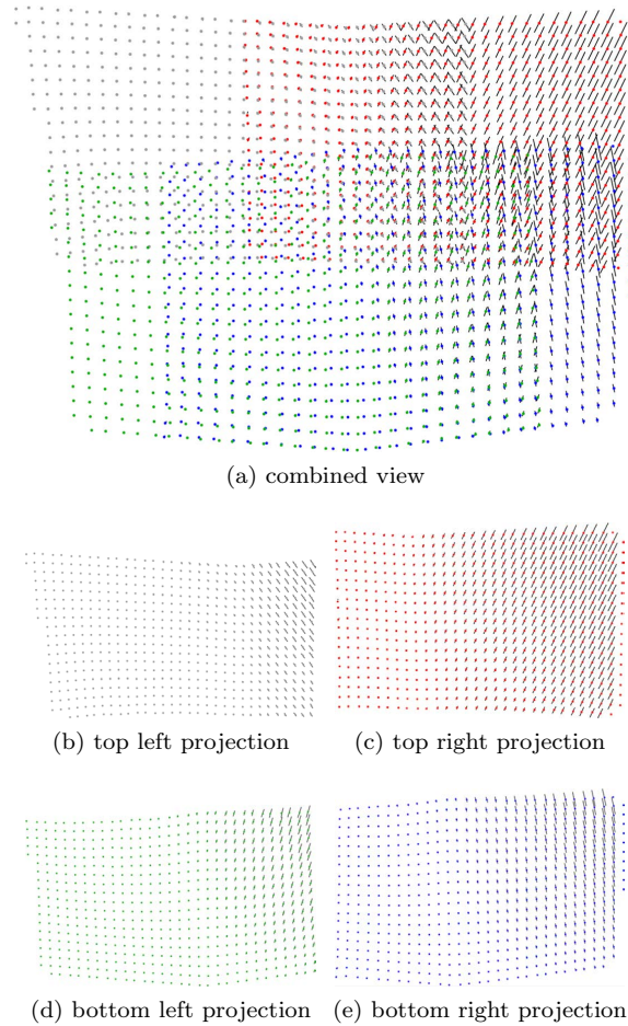
Figure 6.4: A combined view (a) of the linear grid variance shows the configuration (1, 0, 1, t, 1, 0) . By reducing t (i.e., moving one of the actuators), the grid points move towards the top right corner. The dots represent the grids for t = 0.5 , whereas the black line segments denote the connection between the values t = 0 and t = 1 . Viewing the individual grids (b,c,d,e) reveals that the points travel linearly on their segments.
