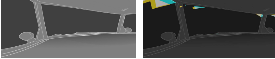
Figure 6.11: In order to optimize the display arrangement, their visibility has been analyzed using cylindrical renderings from the driver’s position (left). The result of the optimization routine (right) consists of the occluding vehicle geometry and displays (rendered in black), and the environment (rendered in cyan and yellow for each eye separately). For ease of understanding the geometry (left) is overlaid semi-transparently.
