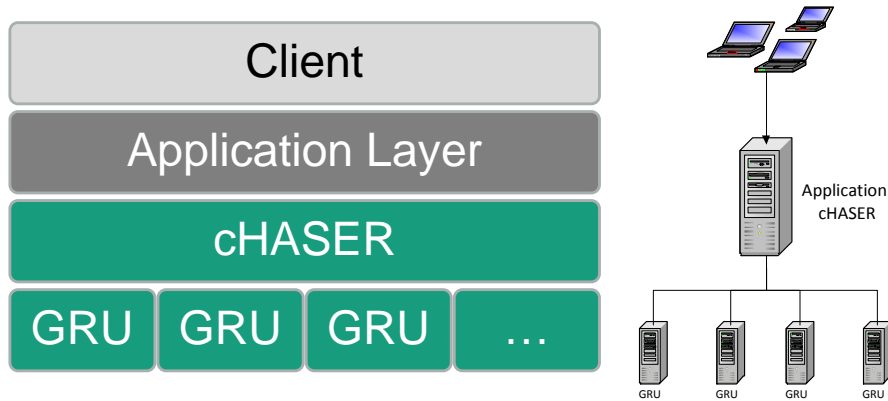
Figure 3.20: The system architecture consist of four layers. Clients are communicating with an application layer representing the generative domain. The main component of the architecture is the cHASER layer for controlling the workload for the GRUs, which are responsible for rendering.
