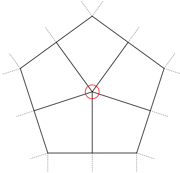
Figure 2.4: A regular mesh of bicubic patches consists of vertices with valence four and is topologically equivalent to an infinite plane, a torus, or an infinite cylinder. To construct different shapes, extraordinary vertices are introduced to the mesh - in this example, a vertex of valence five.
