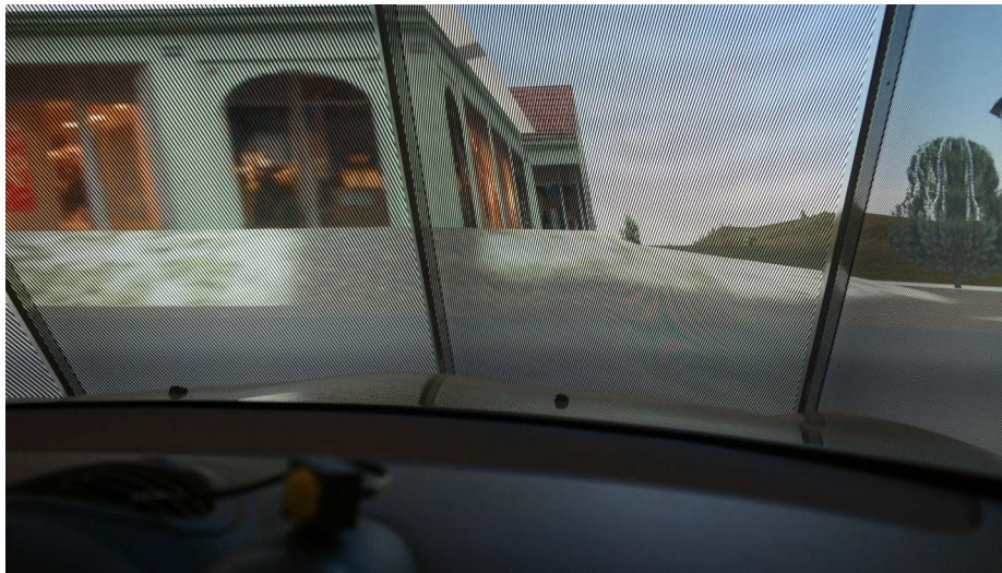
Figure 7.2: The individual parallax barriers for each display are manufactured using acrylic glass. Mounted in precise distance in front of the displays, they are used by the system to separate pixels for left and right eye.
