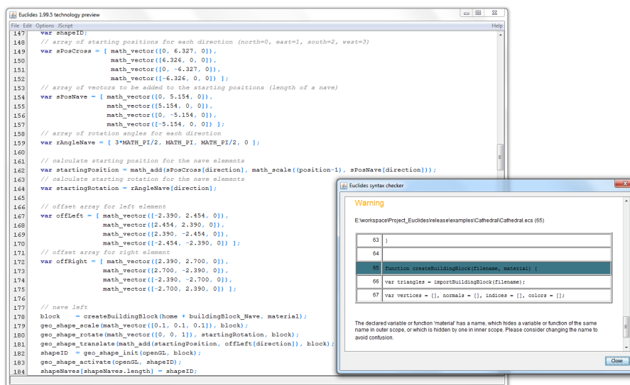
Figure 4.6: The integrated development environment (IDE) consists of a syntax-highlighted editor with line numbers for easy navigation, and a syntax checker with detailed information of warnings and errors.
