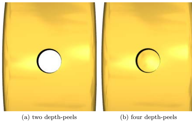
Figure 3.17: Using the correct number of depth-peels shows the back part of the ring as visible through a hole cut into the front part (b). With the number of depth-peels set too low, the back part of the ring is not visible (a).
