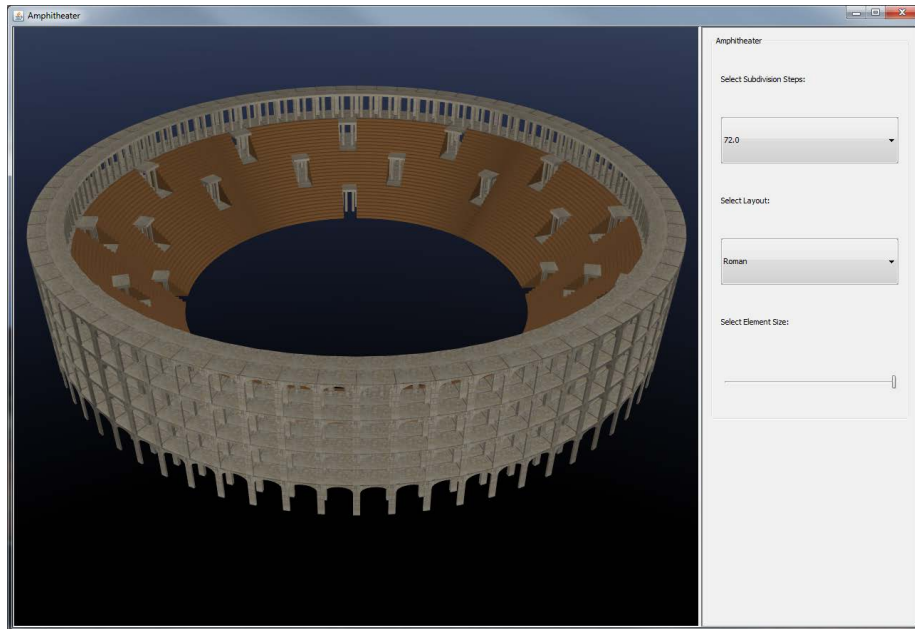
Figure 4.7: The visualization of the amphitheater has been created using Euclides and the Java target. Due to its generative nature and the provided libraries, only 355 lines of code are necessary for the complete example. It is possible to distribute a generative model as an executable JAR file.
