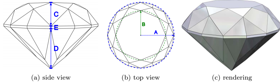
Figure 3.15: Five parameters are used to define the shape of a diamond. The parameters are total diameter (A), table diameter (B), crown height (C), pavilion height (D) and girdle height (E).
