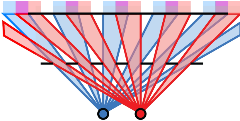
Figure 6.10: The parallax barrier is located between the eyes (visualized in blue and red) and the pixel array of the display. Opaque parts block certain pixels for each eye, while others are visible for one eye only. This results in the eyes seeing only disjoint pixel columns (at least in an optimal setting). If the display is fed with correct image data, the user sees a stereoscopic image.
