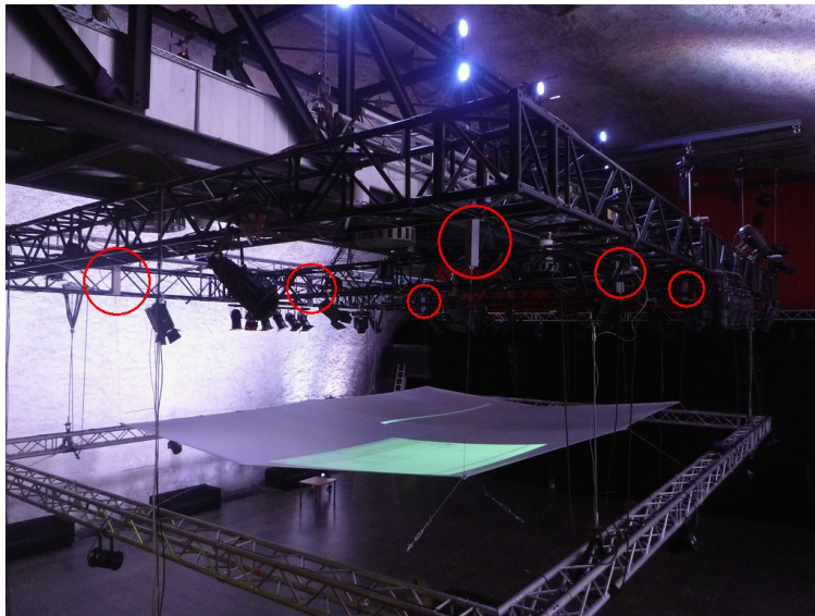
Figure 6.1: The projection setup consists of four projectors projecting onto a movable fabric used as projection surface. It is suspended between electronically controlled actuators (marked by red circles) that can move vertically.
