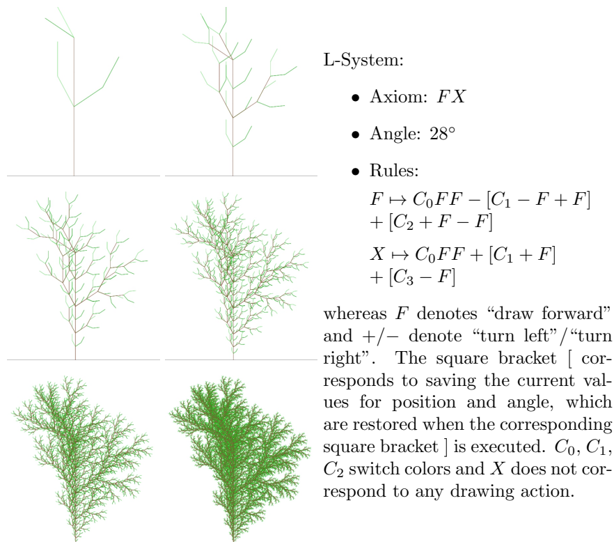
Figure 3.8: Lindenmayer systems are a simple but elegant “turtle rendering” platform. The recursive nature of L-system rules lead to self-similarity and thereby fractal-like forms. Plant models and natural-looking organic forms “grow” and become more complex by increasing the iteration level i.e., the number of substitutions.
