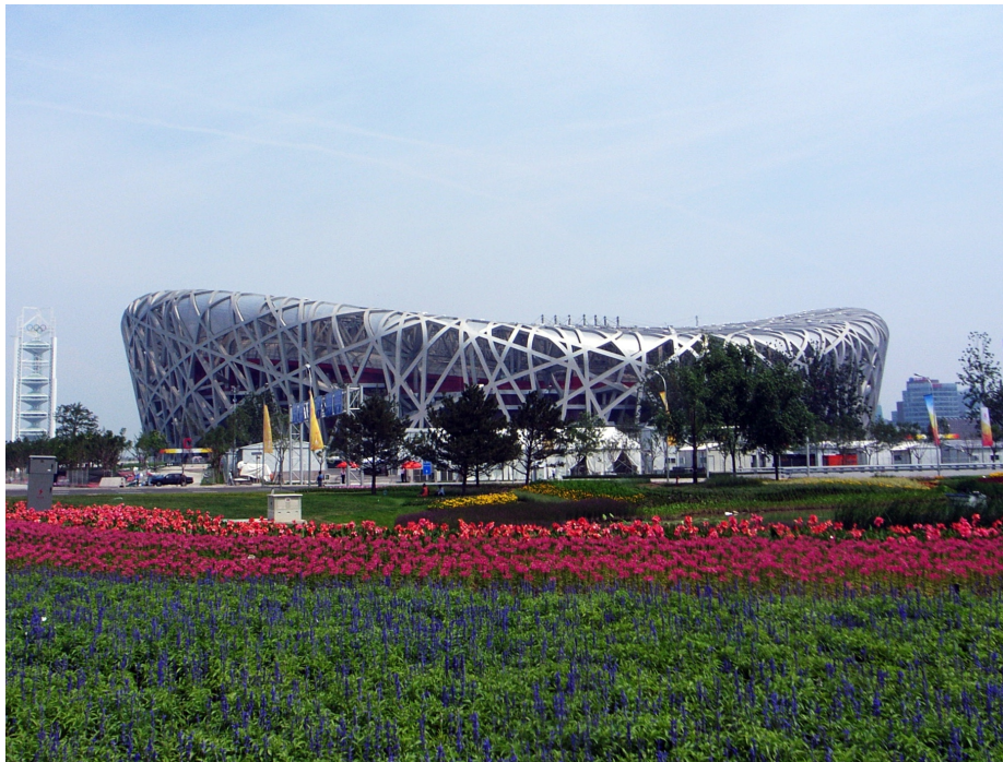
Figure 3.6: The Beijing National Stadium staged the 2008 Olympic Games from 8 August to 24 August 2008. The generative design of its interwoven façade helped saving time in resolving iterations compared to conventional CAD techniques.
