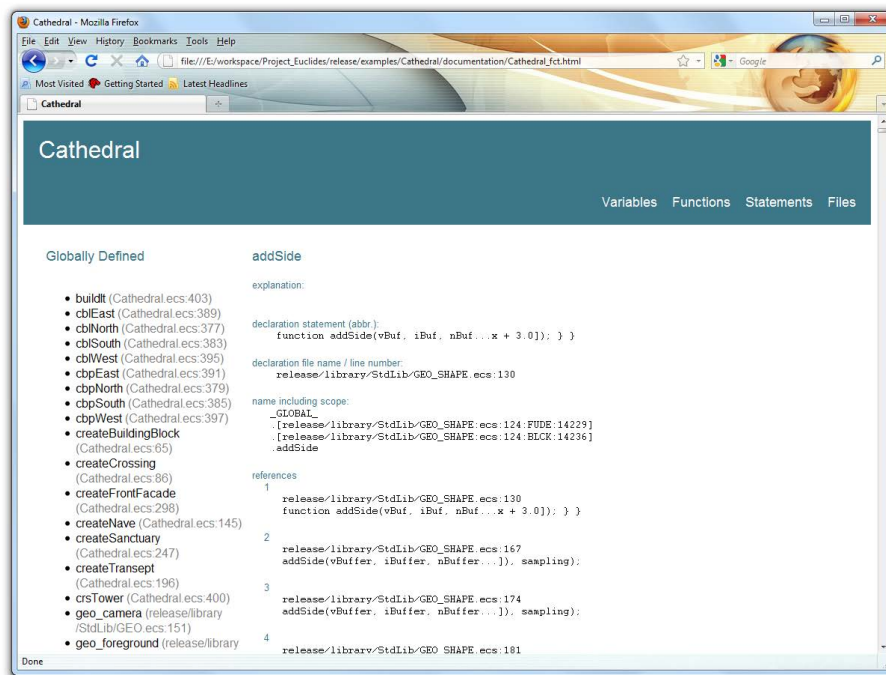
Figure 4.5: The Euclides documentation target, which represents JavaScript as a sustainable, standard-conform XML document can be displayed in an arbitrary web browser.
