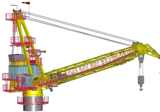
Figure 3.7: The design of ascent assemblies for offshore cranes (colored in red) results in high efforts and causes a major part of the overall engineering costs of a crane. Because of repetitive and nearly identical design processes, the product development processes has been optimized by software driven design automation: the reduction of engineering efforts by modeling design knowledge [Fra11].
