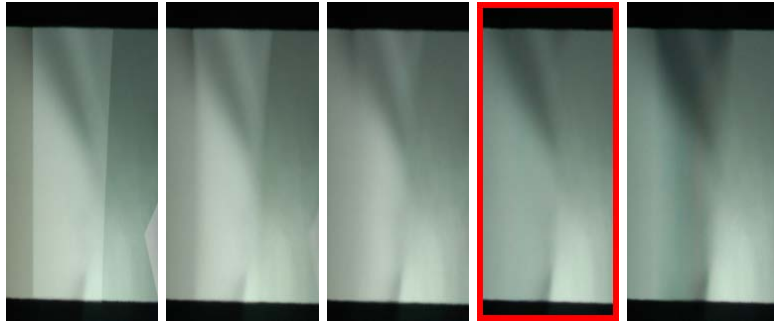
Figure 6.7: Choosing the appropriate projector gamma is essential. From left to right: No blending, blending with \gamma = 0.1 , \gamma = 0.3 , \gamma = 0.6 , \gamma = 0.8 . The correct choice in this case is \gamma = 0.6 .
