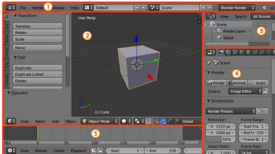
Figure 3.1: The default window of Blender appears. It offers five editors: Info (1), 3D View (2), Outliner (3), Properties (4) and Timeline (5). (Source: Blender Foundation, 2015)
