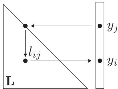
Figure 4.2: If we know the value y_j to be nonzero and l_{ij} is a nonzero as well we know that y_i has to be a (structural) nonzero.
