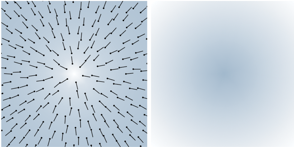
Figure 6.2: Computing geodesic distance using heat diffusion. First the heat kernel is evaluated at a vertex and the piecewise linear gradient is computed (left). Integrating the normalized gradients yields geodesic distances (right).
