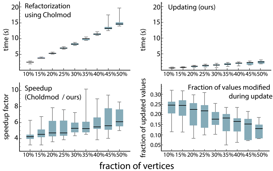
Figure 5.7: Detailed statistics for the Cholesky factor of \mathbf{A}^T \mathbf{A} on a mesh with 5 million vertices. Absolute updating and factorization times across 50 experiments are illustrated (top row) along with the distribution of speedup factors and the fraction of values that need to be updated in \mathbf{L}_{\mathcal{I}} .
