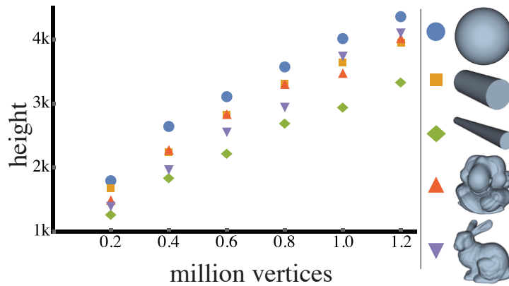
Figure 4.9: The height of the elimination tree for different mesh resolutions, revealing the influence of mesh geometry on performance.
