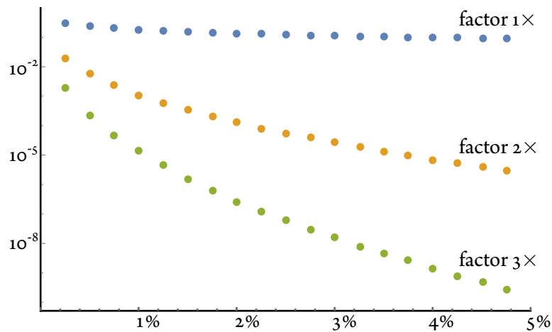
Figure 4.11: The accuracy of the approximate solve increases with the amount of additional values computed.
