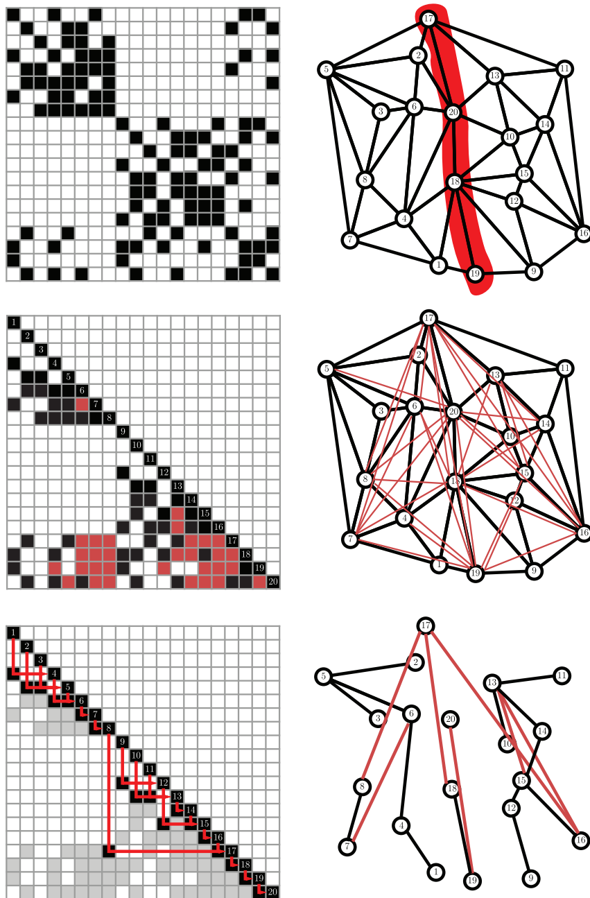
Figure 4.3: The nonzero structure of a discrete Laplacian (upper left) based on the triangular mesh (upper right). The corresponding Cholesky factor contains elements that were zero in the Laplacian matrix (middle), however, because the elimination tree (lower right and Figure 4.4) is nearly balanced, fill in can be limited. A balanced elimination tree will also facilitate fast solving times for sparse and localized sets of vertices.
