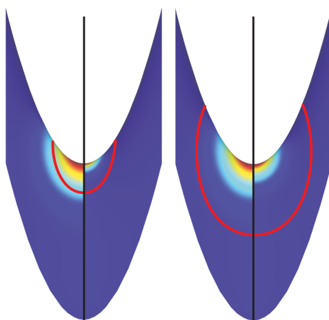
Figure 3.5: The saddle point is correctly identified as centroid for two different cells (red) using heat diffusion. The left side of each image illustrates the sum of squared distances used to define the Riemannian center of mass (3.23).
