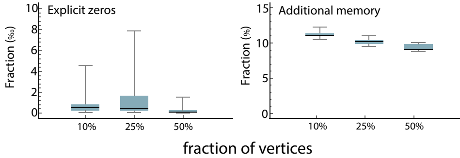
Figure 5.9: Left: The fraction of matrix values that are explicitly stored in our updated factorization although they are actually zero. Right: The amount of extra memory used by our factorization to store additional row information.
