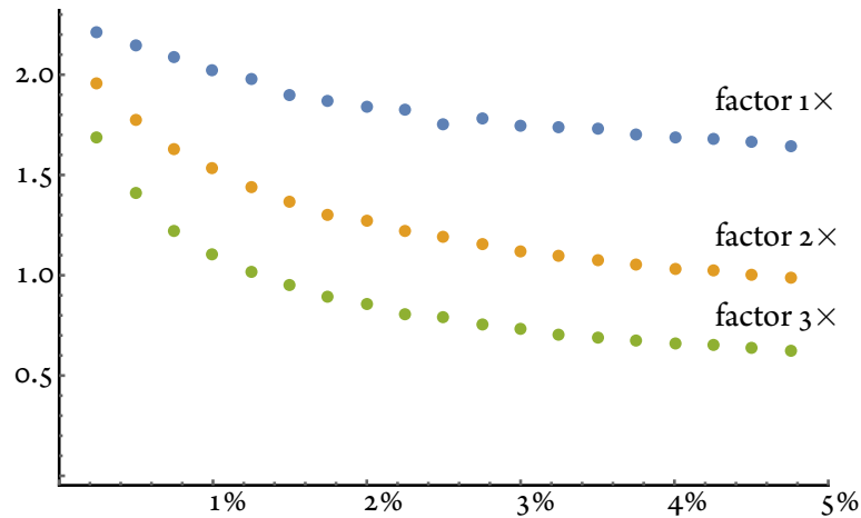
Figure 4.10: Performance ratio of the exact and approximate sparse solve with respect to (circular) patch size (as percentage of all vertices). The radius needs to be enlarged for the approximate method, here we use a factor of one, two and three. Only for patches covering more than 5% of the surface and a factor of > 2 the exact method will be faster.
