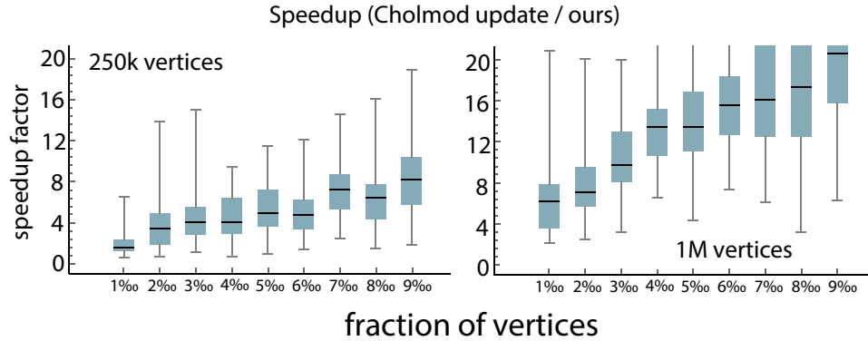
Figure 5.10: Performance comparison of our algorithm and the update procedure implemented in Cholmod. Even for very small meshes and sub-meshes our method outperforms Cholmod significantly.
