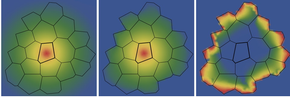
Figure 3.6: The central Voronoi cell is computed using the heat method. The left image shows the heat distribution, the middle image the result of the selective solve, which restricts heat computation to a neighborhood around the cell. The right image illustrates the logarithm of the (relative) distance between the functions. The mean error is 1.8% (max 16%).
