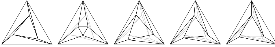
Figure 2.2: The shadow of the Schönhardt polyhedron, a well-known examples for triangular mesh not admitting a perfect Laplacian. From left to right: Original, 1, 5, 10, 50 iterations of our algorithm.
