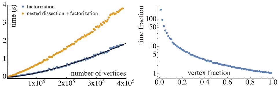
Figure 4.8: Time required for Cholesky factorization and nested dissection (Metis) reordering (left). Time ratio of local patch factorization and factorization time for the full mesh over vertex fraction of the patch (right). Time fraction quantifies how many local factorizations can be computed until it becomes beneficial to compute and exploit a global factorization.
