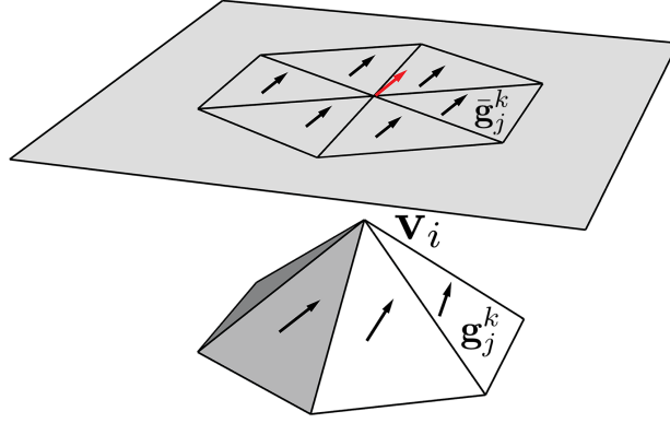
Figure 6.5: Evaluating the gradient of the heat kernel centered at \mathbf{v}_j in all triangles adjacent to \mathbf{v}_i and averaging in the tangent plane gives the angular component of the map.
