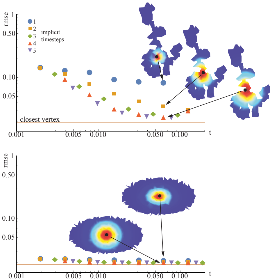
Figure 3.3: The heat center converges to the Euclidean centroid in the plane for large t . The horizontal line represents the distance to the closest vertex, which is the optimum value for the discrete approximation. The effect is non-linear, so requires several linear time steps. For large t the boundary of the finite disk distorts the result. While the non-linearity is clearly visible for irregular polygons (left), Euclidean centroid and heat center are very similar for a wide range of parameters for well-behaved polygons (right).
