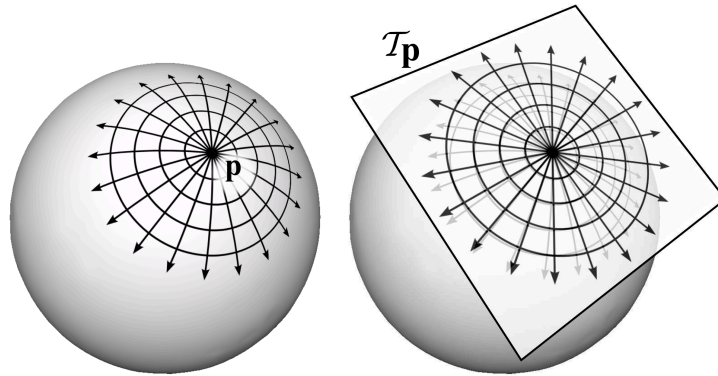
Figure 6.3: Illustration of the exponential map centered at \mathbf{p} . Image courtesy of Ryan Schmidt.
