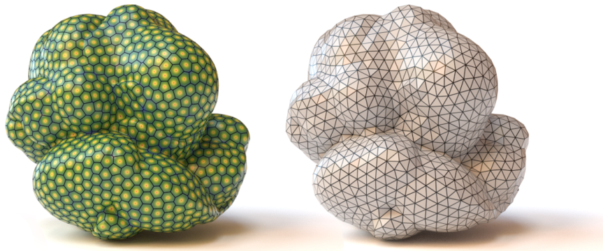
Figure 3.9: Dual Delaunay triangulation of a CVT computed using our Algorithm.
