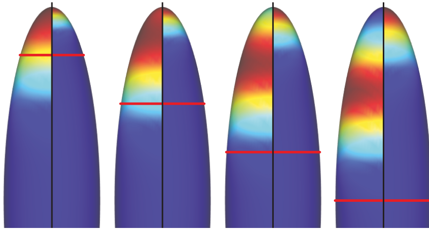
Figure 3.4: The functional defining the center on an elongated ellipsoid. Cells are defined by cutting the ellipsoid orthogonal to the long axis (cell boundaries are marked in red). The left part shows the sum of squared geodesic distances, the right part diffusion values. Color coding is chosen so that the center is in the red area. Already for moderately large cells, geodesic distances become non-unique and the center(s) moves away from the tip. Diffusion naturally defines the tip to be the center.
