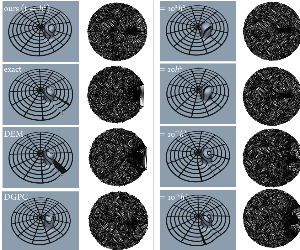
Figure 6.13: Exponential maps in a challenging case including parts of the cut locus. Left: Our method compared to polyhedral geodesics, DEM and DGPC. Right: By varying the time step t of the diffusion problem the smoothness of the map can be influenced. As default choice we use the squared mean edge length h^2 as suggested by Crane et al. [17]. For smaller time steps the exponential maps become similar to the result using exact polyhedral geodesics but are smoother.
