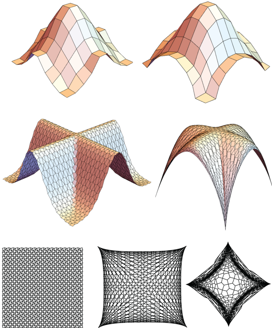
Figure 2.4: Fitting of self-supporting surfaces to several polygonal meshes. The last row shows the planar projection of the input mesh above, the projection of the self-supporting surface and its dual.
