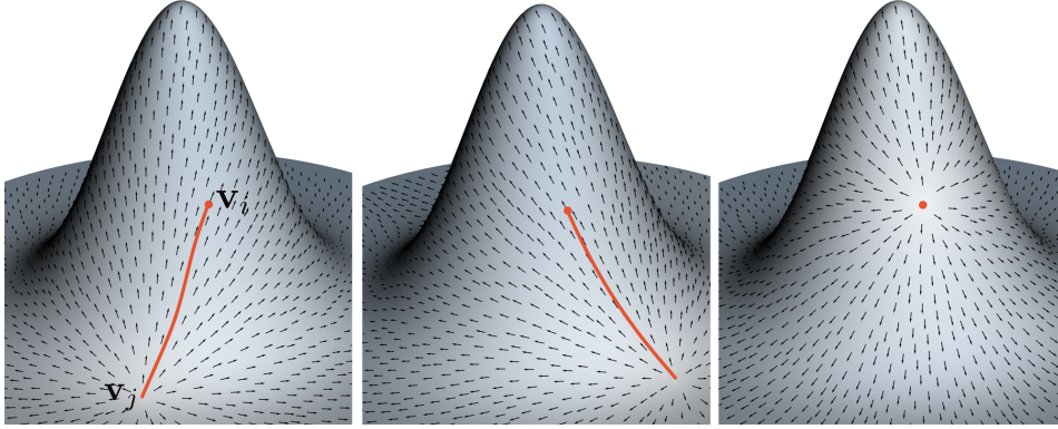
Figure 6.4: Left: Simulating heat diffusion starting at vertex \mathbf{v}_j we obtain tangent vectors to geodesics passing through \mathbf{v}_j . Evaluating these vectors at \mathbf{v}_i defines the angular component of the log map centered at \mathbf{v}_i . Right: We show that in order to evaluate tangent vectors at \mathbf{v}_i for all vertices in a region it is enough to solve only a few diffusion problems close to the center of the map.
