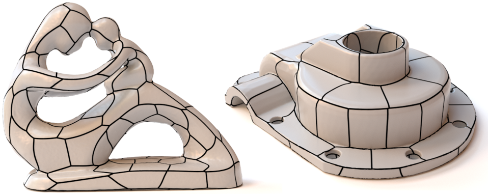
Figure 3.10: Intrinsic Voronoi diagrams enable interesting applications. Anisotropic CVTs are generated by immersing the surface into \mathbb{R}^6 using positions and normals. For non-convex surfaces, this leads to self intersections. The Voronoi diagram on the Klein bottle has been computed in \mathbb{R}^3 , where no embedding of the surface exists.
