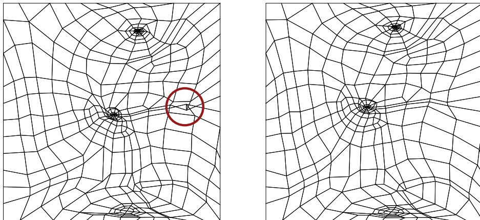
Figure 2.5: Our algorithm produces self-supporting surfaces comparable to state of the art methods. The input mesh (top, left) is deformed towards a self-supporting surface by our method (top, right), the method by Vouga et al. [104] (bottom, left), and using the technique of de Goes et al. [24].
