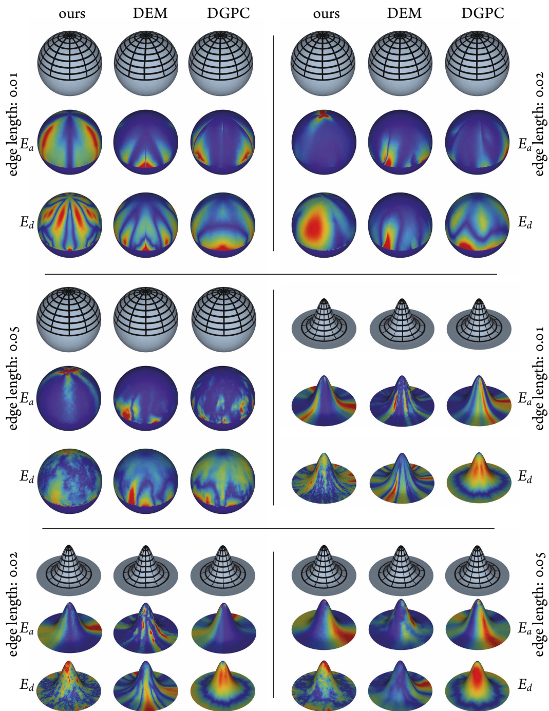
Figure 6.14: Comparing our method, exact polyhedral geodesics, DGPC and discrete exponential maps on basic geometries. The map and errors in angle ( E_a ) and distance ( E_d ) are visualized for different mesh resolutions.
