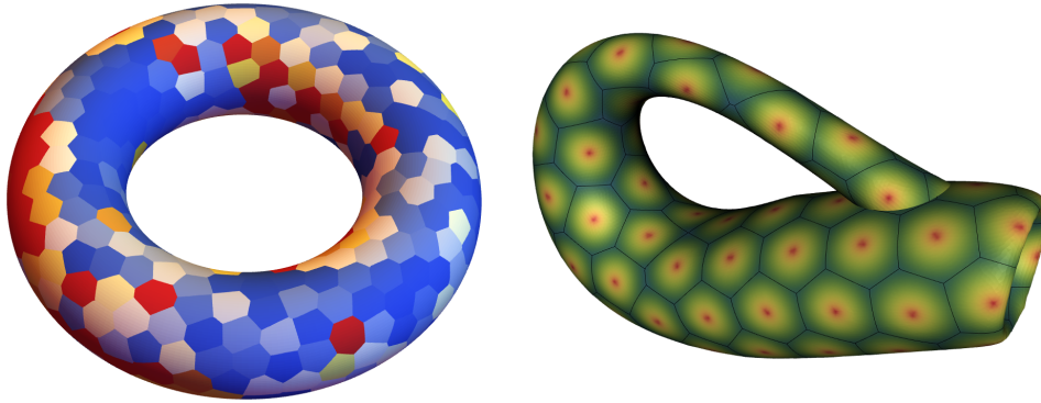
Figure 3.8: Left: the accuracy of our method is not systematically affected by curvature variation. Right: Our fully intrinsic approach enables the computation of Voronoi diagrams and centroids on surface that can not be injectively embedded.
