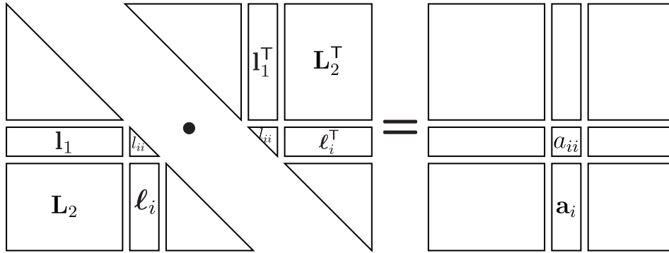
Figure 5.3: Schematic illustration of the left-looking Cholesky algorithm. The algorithm subsequently computes the columns \ell_i by using already computed values to its left in the factor.
