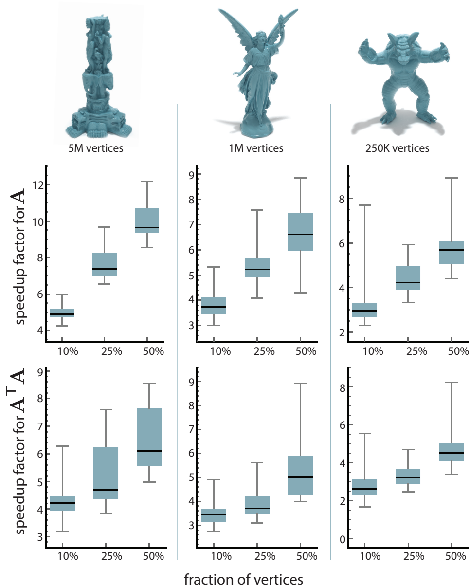
Figure 5.6: Speedup factor of our update method compared to refactorization using Cholmod. The plots show the total range and quartiles for updates consisting of 10%, 25% and 50% of all vertices on three different meshes. Each experiment has been repeated 50 times for the mesh Laplacian A (upper row) and A^T A (lower row).
