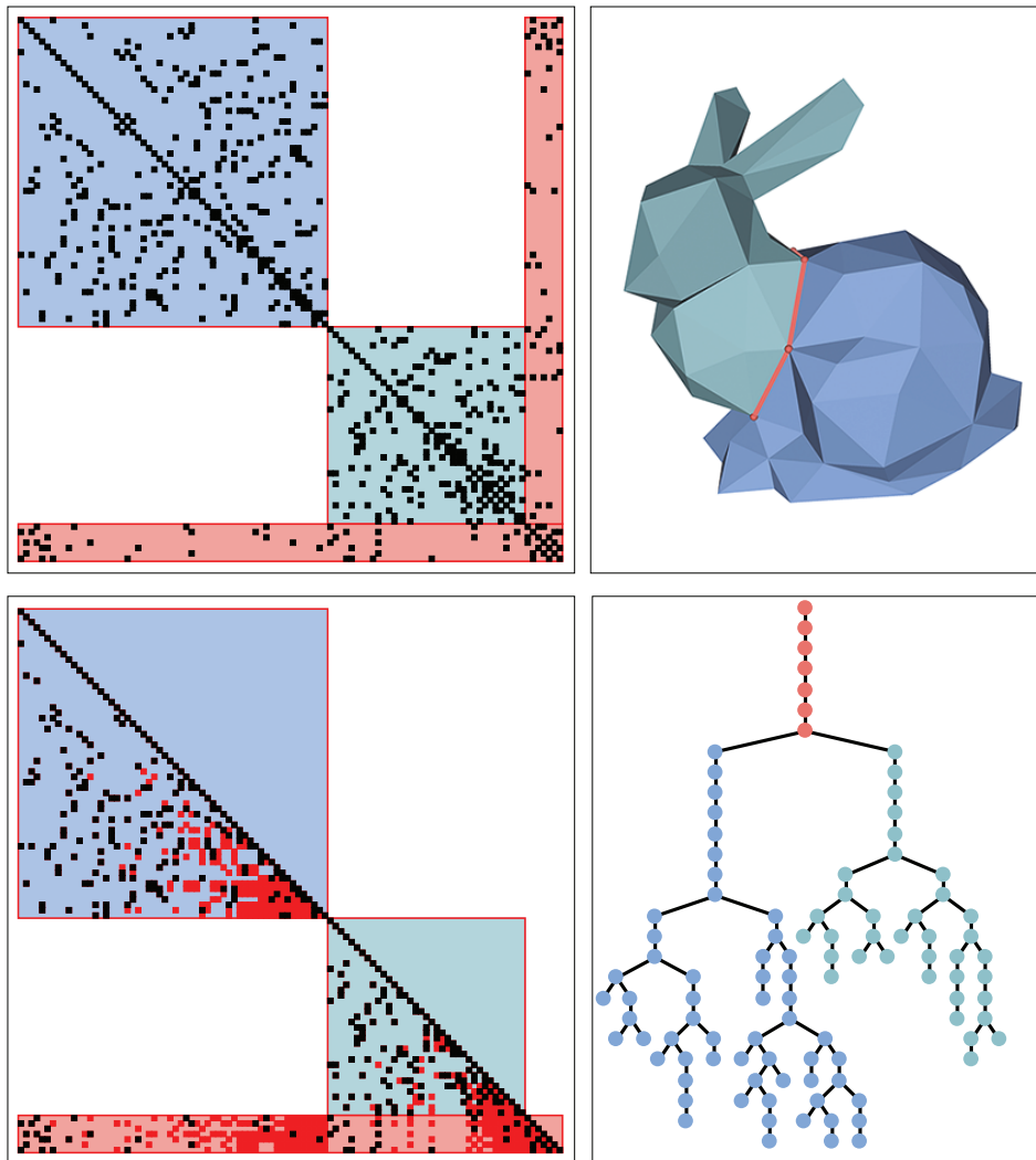
Figure 5.2: Nested dissection reordering hierarchically divides the mesh into two balanced parts separated by a small divider (top right). The mesh Laplacian will then exhibit a block structure (top left). These blocks are preserved in the Cholesky factor (bottom left) which has additional nonzero entries only inside these blocks (red pixels). The block structure yields a fairly balanced elimination tree (bottom right).
