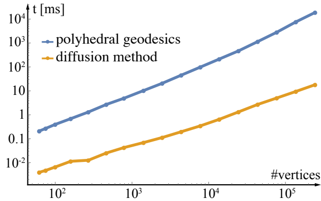
Figure 3.2: Computing the exact polyhedral distance from one points to each other using the algorithm of Qin et al. [80] takes orders of magnitudes longer than computing heat diffusion given a prefactored matrix. This is true for a range of mesh sizes.
