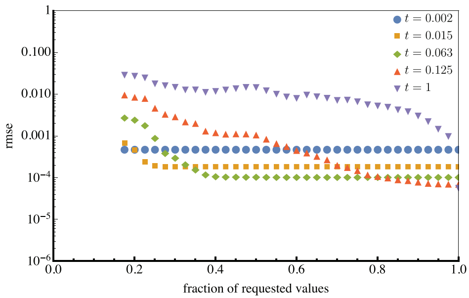
Figure 3.7: Using the approximate sparse solve introduces error which depends on the neighborhood for which values are requested and the diffusion time parameter t .
