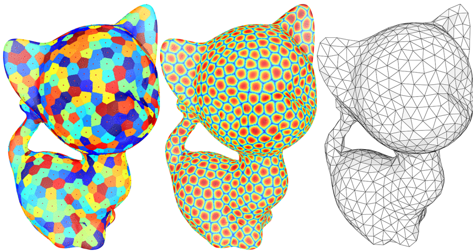
Figure 3.13: Meshing a point cloud by generating a CVT followed by dualization.
