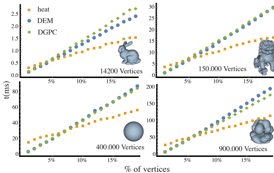
Figure 6.6: Performance for exponential maps using our method ( heat ), discrete exponential maps (DEM) [86] and discrete geodesic polar coordinates (DGPC) [71]. We compare timings for fixed meshes and varying patch size (measured in fraction of total vertices). Each measurement is averaged across 50 random patches.
