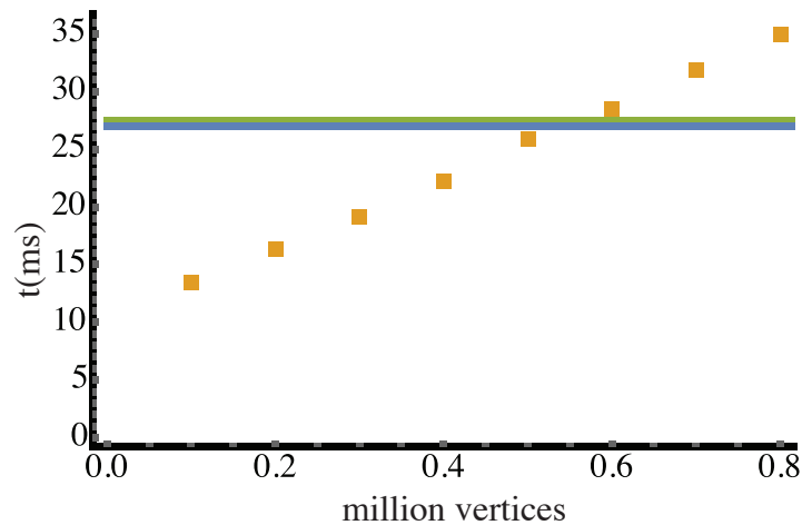
Figure 6.7: Keeping the patch size fixed at 25000 vertices we vary the resolution of the full mesh. Left we see the performance of the heat method (yellow) which can beat DEM (blue) and DGPC (green) if the patch size is below 5% of the full mesh. Consequently we see our method outperform its competitors for meshes with fewer than 5 \times 10^5 vertices.
