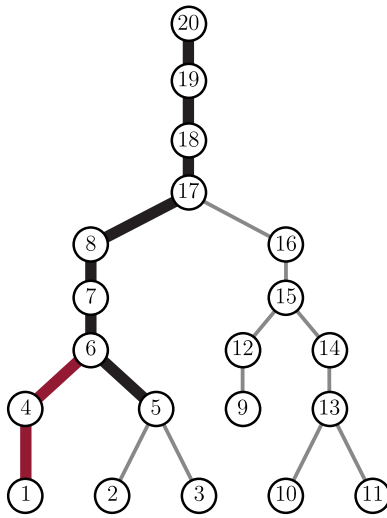
Figure 4.4: The elimination tree of the factorization depicted in Figure 4.3. Having a nonzero at vertex 5 on the right-hand side \mathbf{b} will result in all nodes on the bold black path to become nonzero in the intermediate vector \mathbf{y} . An additional nonzero at vertex 1 will only add vertices on the red path to this set.
