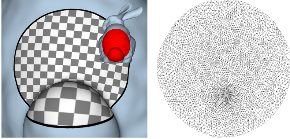
Figure 4.5: A surface patch parameterized using localized harmonic parameterization.
