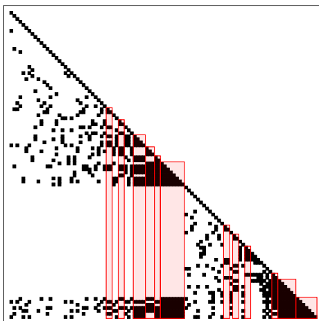
Figure 5.4: Cholesky factors commonly include consecutive columns that share the same nonzero pattern (excluding the diagonal), here shown as red blocks. Aggregating these columns and storing the row information only once is known as the supernodal compressed column representation.
