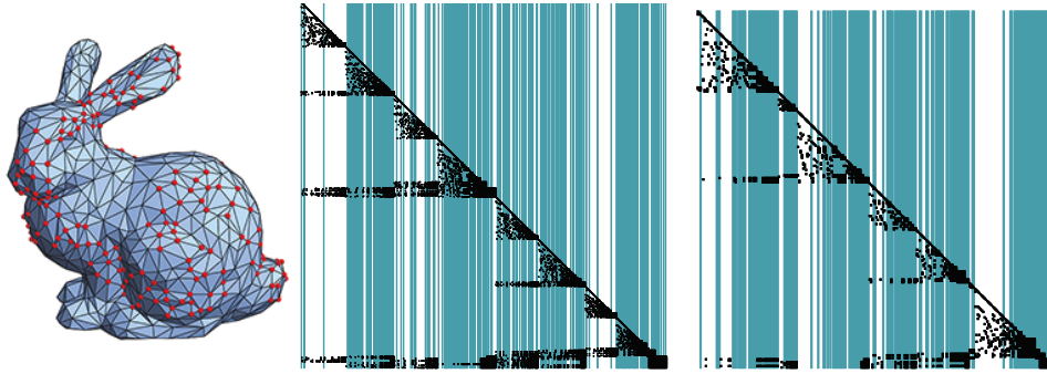
Figure 5.11: Non local patches (left) will induce sub-factors \mathbf{L}_{III} collecting data from many different sub-trees of the elimination tree of \mathbf{L} (center, columns in \mathcal{I} colored) and consequently require costly updates of \mathbf{L}_{III} (right, columns requiring an update are highlighted).
