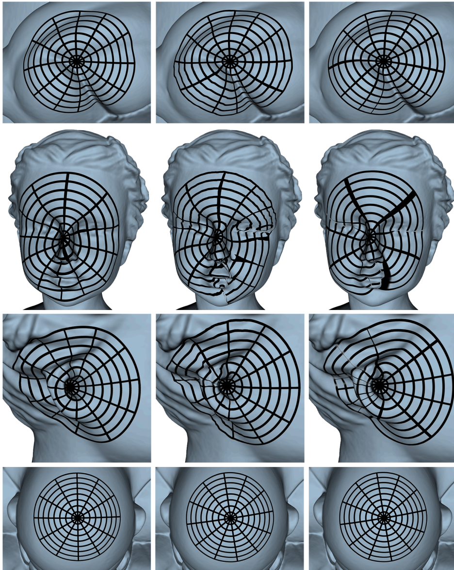
Figure 6.8: Quality comparisons for our method (left), DEM (center) and DGPC (right). Our method yields smoother results for regions of high curvature. For smooth regions all methods perform similar.
