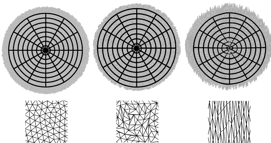
Figure 6.12: Influence of mesh quality on accuracy. Our method performs well also for irregular (center) and anisotropically scaled meshes (right).
