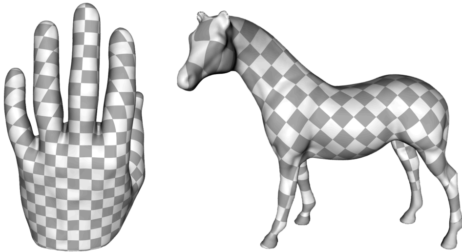
Figure 6.10: Our exponential maps extend smoothly across the whole surface except for the cut locus.
