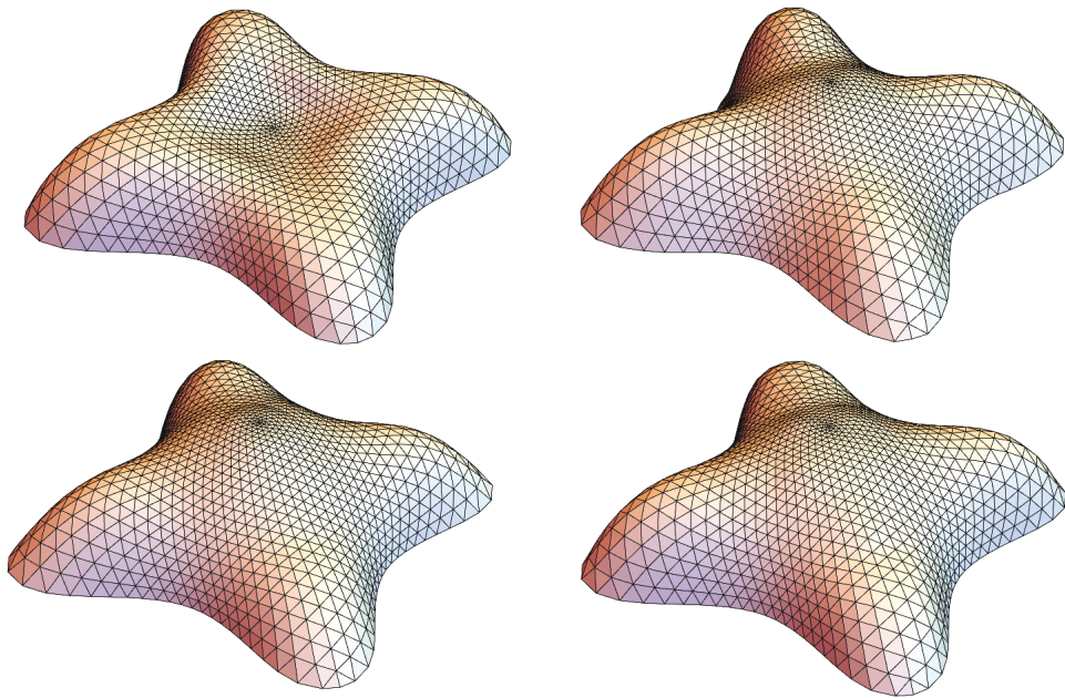
Figure 2.5: Our algorithm produces self-supporting surfaces comparable to state of the art methods. The input mesh (top, left) is deformed towards a self-supporting surface by our method (top, right), the method by Vouga et al. [104] (bottom, left), and using the technique of de Goes et al. [24].
