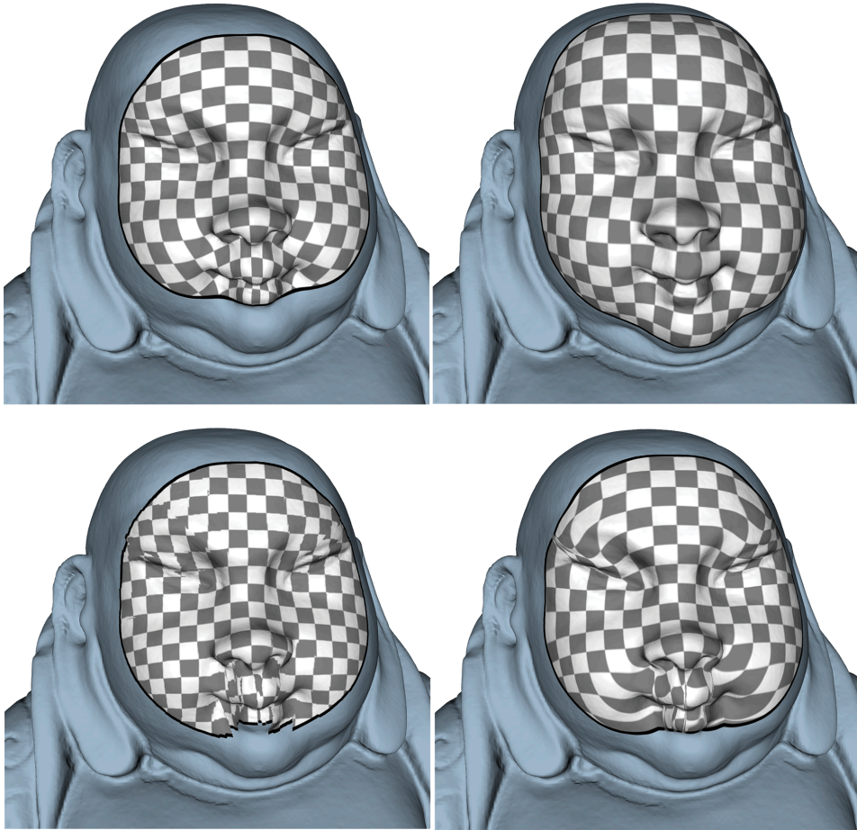
Figure 6.9: Comparison of our method (top left), conformal map (top right), DEM (lower left) and DGPC (lower right).
