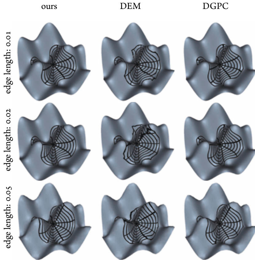
Figure 6.11: Exponential maps at a saddle point for meshes of different resolution.
