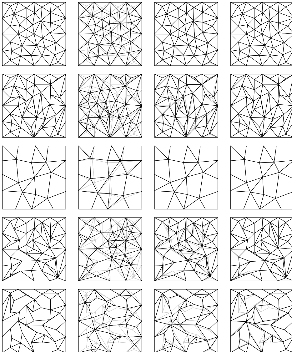
Figure 2.1: Results created by our approach for different classes of polygon meshes. Each row depicts iterations of our algorithm starting with an input tessellation.
