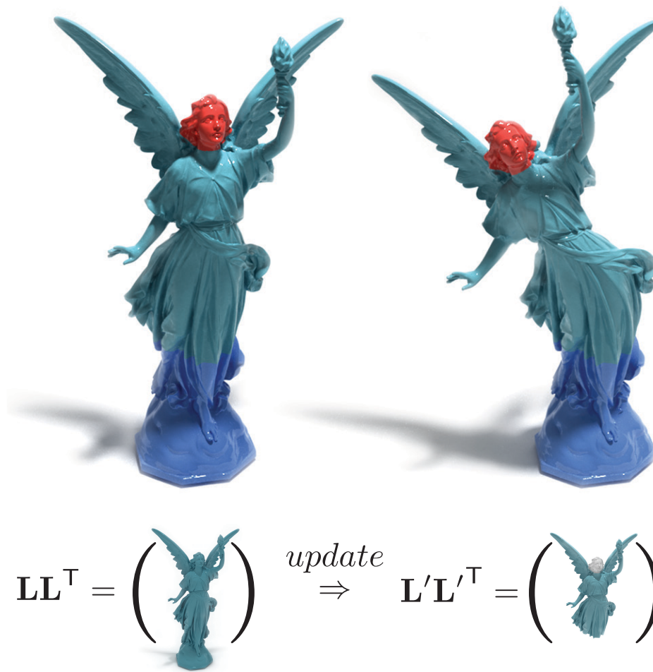
Figure 5.1: Deforming a mesh based on selecting a region of interest (green) and a handle (red) commonly requires solving a sparse linear system. This is typically done using the Cholesky factorization. The computation time for the factorization depends on the number of vertices in the region of interest, and may prohibit interactive use for large meshes. We propose a method that exploits the factorization of the operator \mathbf{L} on the whole mesh for computing the new factorization of \mathbf{L}' on the submesh, instead of computing it from scratch. For the depicted mesh with one million vertices our update algorithm computes a new factorization in 0.47 seconds whereas the factorization of the desired system matrix for the region of interest using Cholmod takes 3.4 seconds.
