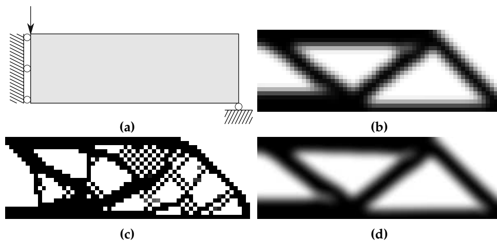
Figure 2.20 – Illustration of the checkerboard problem. (a) Boundary conditions of the classical MBB problem. (b) Low-resolution solution, using a 60 \times 20 grid and a density filter with radius 2.4. (c) Low-resolution solution without filtering. (d) High-resolution solution, using a 300 \times 100 grid and a density filter with radius 12 (which corresponds to 4% of the domain width).
