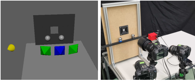
Figure 3: Schematic overview (left) and realization (right) of the scanning setup featuring one main camera (blue) and two side cameras (green) for light source estimation from two mirror balls. A handheld flashlight (yellow) illuminates the skin which is pressed against a small cutout window from the back.
