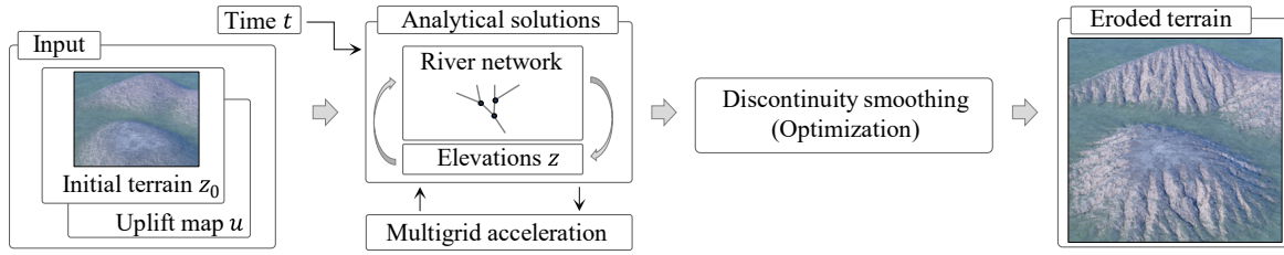
Figure 2: From a user-provided initial terrain z_0 , uplift map u , and target time t (left) our method outputs the eroded terrain at time t . Contrary to simulation-based approaches, our algorithm does not rely on a time-stepping scheme but uses the analytical solutions of the stream power law. To compute these solutions, we rely on a multi-grid accelerated process that iterates over both the computation of the river networks and the computation of the elevations predicted by 1D analytical solutions embedded in these rivers (center left). Optionally, the user can choose to interrupt this iteration before convergence, for example, to preserve the initial river network, and in this case, we propose an optimization-based approach to smooth the remaining discontinuities (center right).
