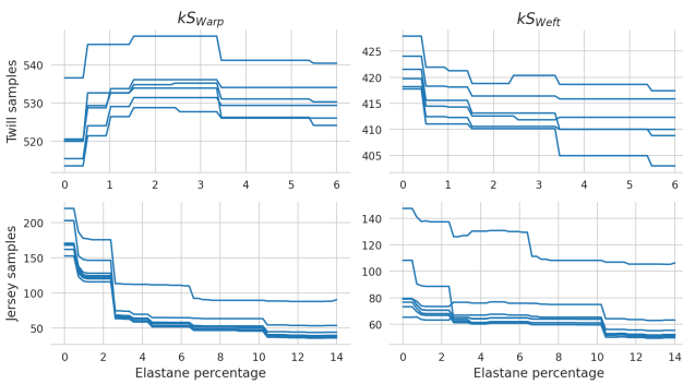
Figure 10: Effect of changing elastane percentage of randomly sampled dataset jersey and twill fabrics on the output mechanical parameters. As elastane increases in jersey fabrics, the resistance to stretch is decreased in warp and weft directions, but more notably in the warp direction. A different effect is observed in the case of twill fabrics, for which the stretch resistance decreases only in the weft direction.
