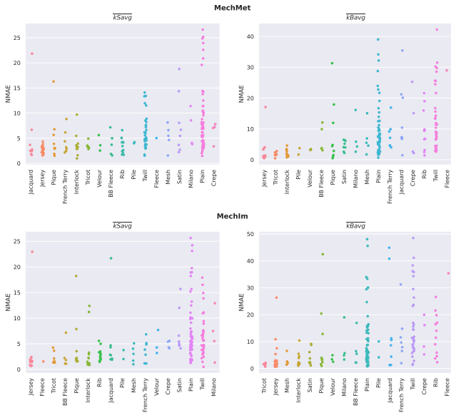
Figure 7: Normalized kS_{avg} and kB_{avg} errors of all the fabrics per family, sorted by increasing median family error.
