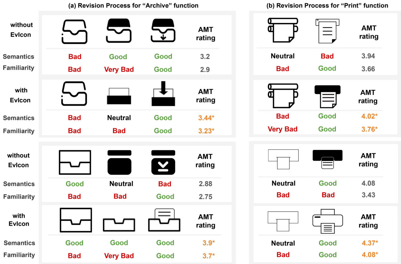
Figure 10: Icon revision process starting from left to right by designers with and without EvIcon. (a) presents the revision processes for 'Archive' icons of two designers, and (b) presents the revision processes for 'Print' icons of two designers. Eight groups of revision process with the prediction of perception feedback and the crowdsourced evaluation results ('AMT rating') of the finalized icons are presented (the better AMT ratings are highlighted with the star symbol).
