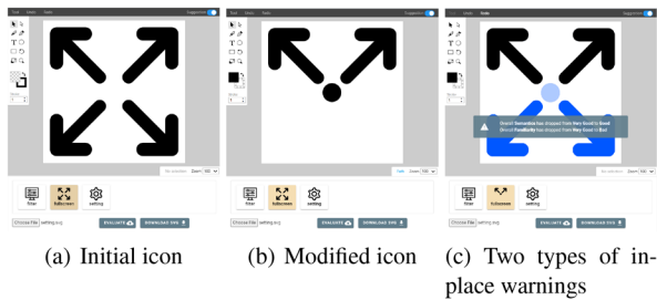
Figure 4: A warning will be displayed in place to draw attention to the poor adjustment compared to the last usability inspection. Blue highlights will indicate the paths suggested to be added back, while light-blue highlights will mark those suggested to be removed.
