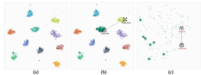
Figure 6: (a) Different colour-codings indicate different semantic concept clusters. The icons are linked (b) in grey but will change (c) to red in order to notify poor visual distinguishability.
