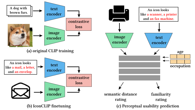
Figure 7: (a) The general-purpose CLIP [RKH*21] is a joint image-text embedding trained on 400 million text-image pairs. (b) We fine-tune the general-purpose CLIP into IconCLIP using 'icon tags'-'icon image' pairs. (c) We predicted the perceptual usability ratings of an input icon and its associated tags using the IconCLIP embedding space and the target demographic information.
