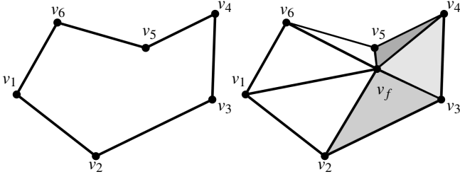
Figure 3: Spanned triangle fan on the virtual mesh after inserting the vertex v_f . The figure was taken from [BHK20].
