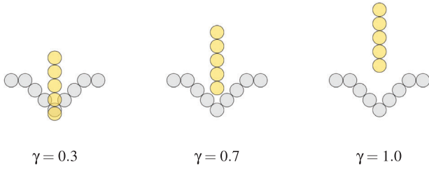
Figure 2: An illustration of the effect of \gamma on the contact detection between two rigid bodies. With \gamma = 0.3 , interpenetrations between bodies may occur since contributions from neighbouring particles might not be enough to detect a collision. This is especially problematic for thin geometry features such as the yellow rod displayed. Setting \gamma = 1.0 causes large gaps between rigid bodies and finer features such as the notch in the grey body is ignored due to the collision between the bodies being detected too early. We achieve the desired result by setting \gamma around 0.7.
