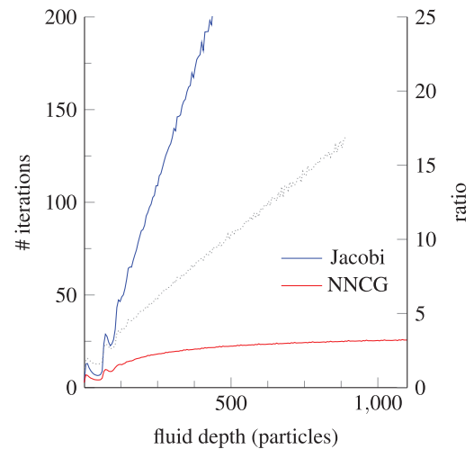
Figure 8: The required solver iterations of the default Jacobi solver (blue) and the NNCG solver (red) in relation to an estimate of the fluid pillar depth in particles. The ratio between the Jacobi iterations and NNCG iterations is indicated as a grey dotted line. Over time, the fluid pillar grows in height and as such the number of required solver iterations increase. We can see that for the Jacobi solver, the required solver iterations increase approximately linearly with fluid depth, while the NNCG iterations only show sub-linear growth. Thus, in the shown scenario, for high fluid depth, the performance advantage of the NNCG solver becomes increasingly significant.
