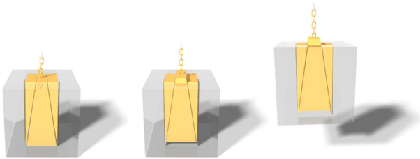
Figure 9: A Lewis lifting mechanism. When pulled upwards, the inner pyramid shaped piece presses the wedges against the outer weight. Solely due to frictional forces, the outer weight is lifted.
