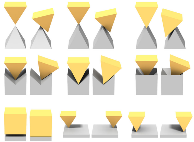
Figure 5: Degenerated test cases proposed by Erleben [Er18] which can be challenging for mesh-based contact handling methods. For each of the nine constellation, we show the initial setting and right next to it a snapshot of the simulation. The bodies are given some initial velocity as described in Erleben [Er18]. Visually, our particle-based contact handling shows no problems whatsoever when simulating the shown constellations.
