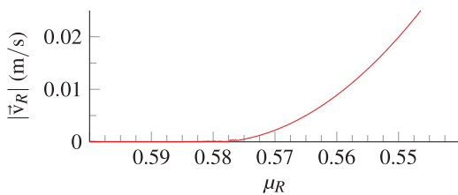
Figure 4: The relation between the coefficient of friction \mu_R of rigid body R and the magnitude of its translational velocity \vec{v}_R using our friction model. We can see that R starts accelerating as soon as \mu_R < 0.577 which is in good agreement with the analytical solution. Note that the velocity increases in a quadratic manner as \mu_R decreases.
