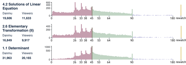
Figure 7: Behaviors comparison in different videos. The first two videos have very similar behavior distributions. They both have more time_less behaviors with the angle below 26^\circ .
