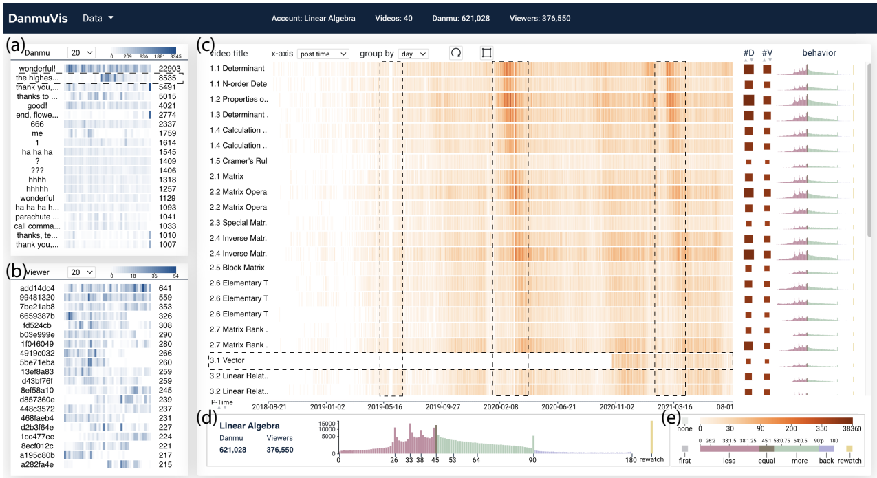
Figure 4: The video corpus exploration interface supports danmu analysis across different videos. Top danmu comments are listed in the comments view (a), while the viewers view (b) displays active viewers in the video collection. The videos comparison view (c) compares metrics of danmu in different videos against the selected time dimension (post time). The behavior statistic view (d) shows the behaviors information of the video corpus. The legend view (e) demonstrates the color encoding method of the interface. For the convenience of non-Chinese readers, danmu texts and video titles are translated from Chinese to English.
