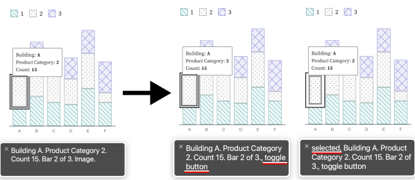
Figure 5: An interactive chart displaying only “Image” as semantic information with no feedback provided on selection. The robust semantics given to a screen reader, “toggle button” (middle) as well as instant feedback, “selected” (right) are considered proper semantics for an interactive experience.
