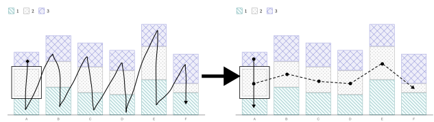
Figure 2: Keyboard navigation paths on a stacked bar chart. The left shows a serial navigation example, typically just a default of rendering order. The right shows both groups (the stack of bars) and categories (the color/texture shared among bars across stacks) as dimensions to explore laterally or vertically.
