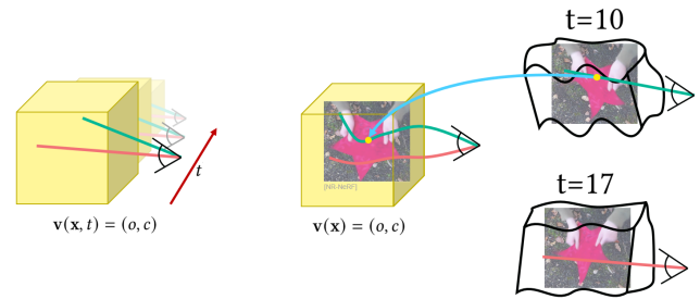
Figure 8: Current methods for modelling deformations with neural radiance fields fall into two categories. Left: Implicitly, by conditioning the radiance field, \mathbf{v} , on the deformation (here: time t ). Right: Explicitly, by warping space with a separate deformation MLP that regresses offsets (blue arrow) from the deformed space (black) into static canonical space (yellow). This bends straight rays into the canonical radiance field. Image adapted from [TFT*21].
