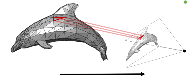
(a) Forward Rendering (e.g., rasterization) – the image is generated by projecting the 3D representation to the image plane.
