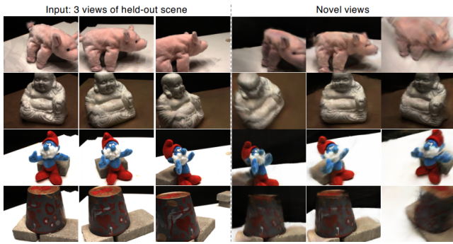
Figure 7: Input images from DTU MVS dataset [JDV*14] and novel views obtained by PixelNeRF [YYTK21] with no test-time optimization. Furthermore, training and test sets do not share the same scenes. Image adapted from [YYTK21].
