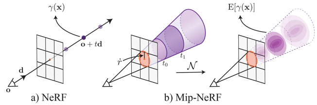
Figure 6: Instead of sampling points x along the rays traced from the camera projection center (a), MipNeRF [BMT*21] reasons about 3D canonical frustum per camera pixel (b). Image adapted from [BMT*21] ©2021 IEEE.
