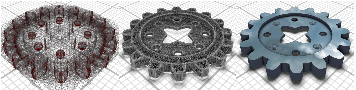
Figure 1: Our method takes a CSG object defined by quadric surfaces and computes a set of per-surface low-distortion parametrizations. On these, we perform an adaptive subdivision guided by a conservative distance function (left). Once all CSG surface patches are identified, we can generate point samples on them (middle). Our splat-based rendering guarantees perfect surface reconstruction (right). In this example, 327 000 samples across 80 quadric primitives were generated. For models of this complexity, we can generate about a million surface samples per second per CPU core. Render time is 0.5 ms at 1080p.
