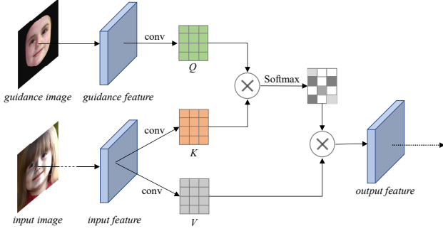
Figure 3: Transformer block.
