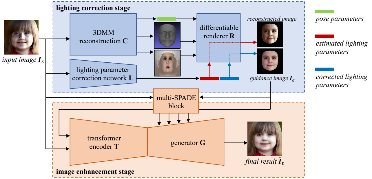
Figure 2: The schematic illustration of our method.
