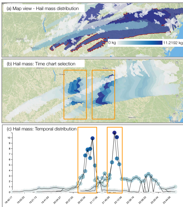
Figure 11: (a) Hail mass development during the tornado outbreak, March 3rd, 2019. (b) Analysis of hail mass in a thunderstorm. Several independent branches joined and converged into a big structure. (c) Temporal evolution of the selected thunderstorm showing two peaks with high concentrations of hail mass.
