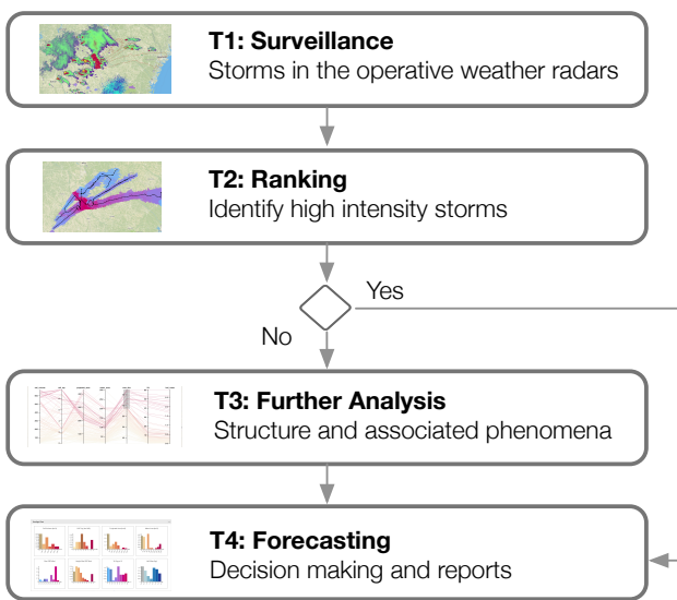
Figure 2: Hornero's tasks workflow adapted from the domain experts' feedback and task workflow.
