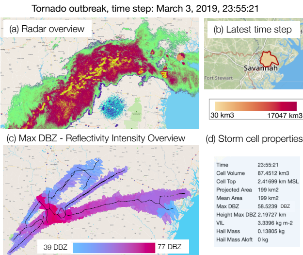
Figure 9: Thunderstorm that extends towards Florida’s coast near Savannah. An overview of the radar data for the latest time step (March 03, 2019 23:55:21) can be seen. (a) the radar reflectivity corresponding to the selected time step, (b) the storm cell detected by Titan at the selected time step, (c) the complete reflectivity intensity evolution (max dbz), and (d) the storm cell properties.
