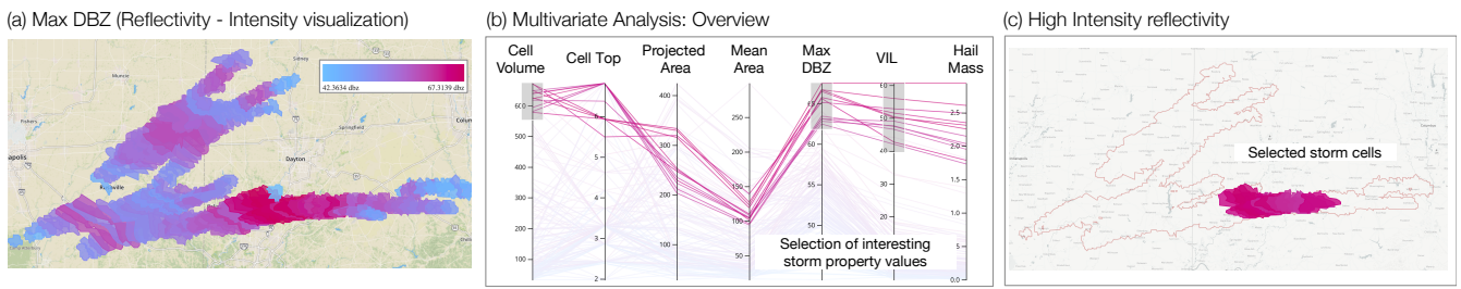
Figure 5: Using the Characteristics view (b), forecasters can filter storms to analyze the May 27, 2019 outbreak. The left plot (a) shows a storm intensity overview (Max_DBZ). (b) shows the selection of cell volume, intensity (Max_DBZ), and VIL for filtering potentially dangerous storm cells. The right plot (c) shows the resulting query on the map by brushing on the Characteristic view.
