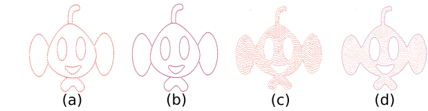
Figure 3: Two common types of inputs to the 2D reconstruction algorithms. (a) Boundary sample (b) Reconstructed curves (c) Area sample (d) Reconstruction from area samples.
