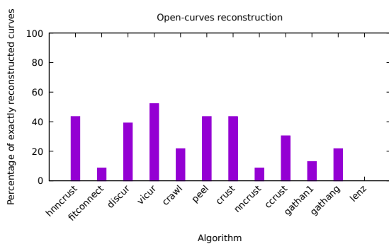
Figure 19: Percentage of exact reconstruction of open curves by different algorithms. We tested the algorithms on 23 different open curves collected from various curve reconstruction papers (run-open-curves.sh).
