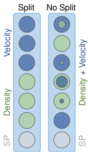
Figure 4: Visualization of a LS with |\mathbf{c}| = 7 . Using the split loss, we optimally obtain a clear differentiation of the input quantities velocity and density, while their influence is spread across the whole domain using classical training methods as visualized below the No-Split label.
