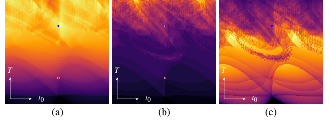
Figure 4: f_{\rho_{\text{len}}} (a), f_{\rho_{\text{cnt}}} (b), and f_{\hat{\rho}_{\text{len}}(k)} (c) aggregation fields, applied to the Quad-Gyre dataset, with \tau_{\lambda} = -0.05 and the same parameters as for Figure 3. Note that (a) shows a rather continuous field, while (b) contains only integer numbers of ridges, and (c) displays a similar structure due to its dependency on the number of ridges. Additionally, while \rho_{\text{len}} increases with T due to longer, sharper ridges, \hat{\rho}_{\text{len}}(k) exhibits in (c), toward higher T values, a sharp drop in the quality of extracted ridges caused by aliasing. The rather noisy top part in all fields shows that the chosen spatial resolution is unable to capture the ridges at high T values well, so they break up in an unpredictable manner causing these patterns.
