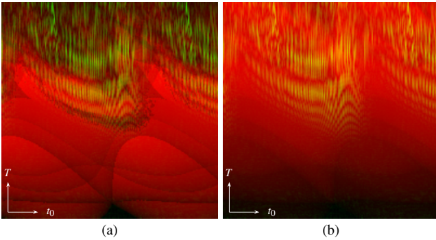
Figure 7: Aliasing aggregation field f_{v_{\text{sum}(2)}} mapped to the green channel, and f_{\rho_{\text{len}(k)}} (a), and f_{\rho_{\text{len}}} (b) mapped to the red channel for the dataset from Figures 4a, 4c, and 6d. Note that in (a), the fields are somewhat complementary because the ridge quality decreases as the aliasing problems increase, whereas in (b), they both show the same increasing trend with T .
