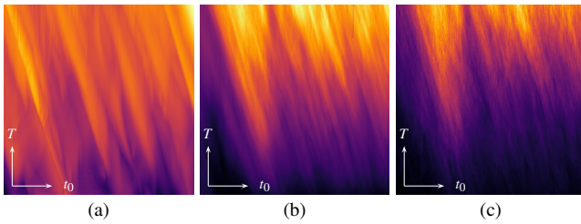
Figure 12: Buoyant Flow dataset with G_{\text{agg}} = 500 \times 500 and G = 400 \times 400 , t_0 \in [0, 0.3] , and T \in [0.01, 0.1] . All fields f_{\sigma_{\text{max}}} (a), f_{\rho_{\text{plen}}} (b), and f_{\rho_{\text{cen}}} (c) show a similar structure with this dataset. The ridge aggregation fields, however, show that the LCS are only sharp enough to be detected as ridges at high T values.
