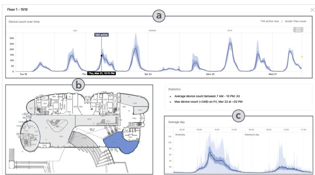
Figure 5: Region detail view. (a) Zoomable binned time series chart. (b) Floor plan for spatial context and navigation. (c) Typical day profiles.
