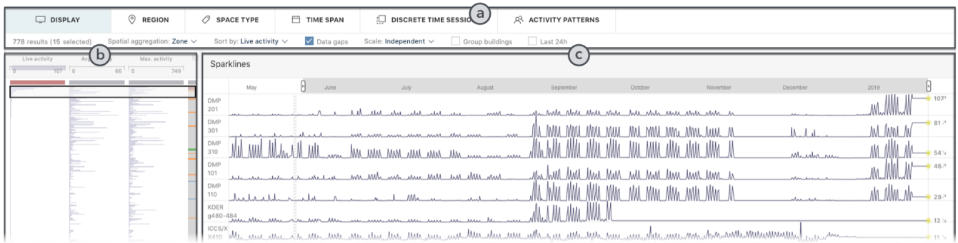
Figure 2: Campus Explorer Interface. (a) Control panel for filter and display settings. (b) High-level region overview shown as quantitative and categorical data stripes. (c) Region subset view providing mid-level details for regions selected in the region overview; users can choose between different visual encodings for it. Clicking on one region opens a modal region detail window with low-level details.
