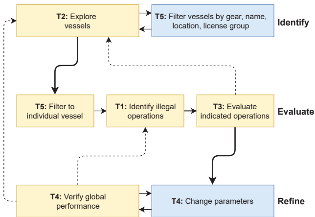
Figure 2: The user's workflow based on abstract tasks. Yellow tasks are mandatory, blue are optional. The flow of user operations is denoted by arrows. The workflow can be grouped into the following three phases. Identify: After automatic analysis, the user identifies vessels of interest, for instance ones with indicated operations. If not looking for a known vessel, the user filters the dataset to focus on a specific subset of vessels. Evaluate: The user verifies whether a single vessel from the subset may have performed an illegal activity by analyzing its trajectory and reports, and comparing these to the results of the indicators. Refine: If unsatisfied with the results of the indicators, the user tweaks indicator parameters, verifies that the global indicator performance is not reduced, and either keeps refining, explores a new set of vessels, or returns to the vessel currently being evaluated.
