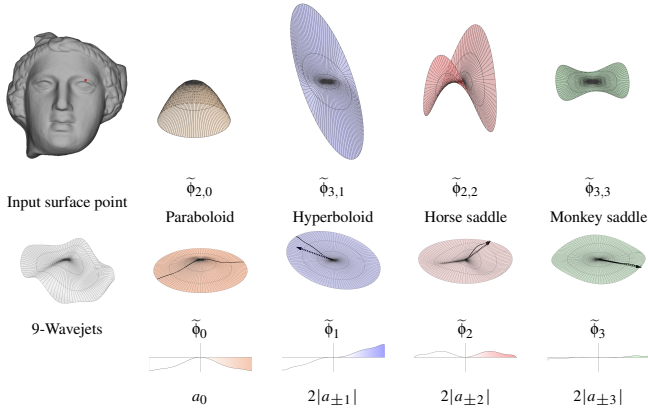
Figure 3: Wavejets decomposition around a point of a surface. Left: approximated 9-Wavejets surface. Let \tilde{\phi}_{k,n}(r,\theta) = r^k (\phi_{k,n}e^{in\theta} + \phi_{k,-n}e^{-in\theta}) and \tilde{\phi}_n = \sum_{k=0}^{\infty} \tilde{\phi}_{k,n} . The amplitude of the functions \tilde{\phi}_n is more comparable to the amplitude of the input surface than the functions \tilde{\phi}_{k,n} .
