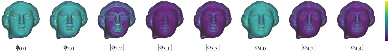
Figure 2: Computation of some values of \phi_{k,n}(\mathbf{p}) for a radius R_\phi corresponding to the height of the eyes of the statue. If k and n do not share the same parity, coefficient \phi_{k,n} is zero. For k \geq 0 and n \neq 0 , only the magnitude of \phi_{k,n} is displayed since the phase depends on the origin direction of the angles. For k \geq 0 , \phi_{k,0} is real, does not depend on the origin direction, and can be negative. Note that \phi_{1,1}(\mathbf{p}) = 0 if the parameterization plane is the tangent plane at \mathbf{p} to the surface. \phi_{0,0}(\mathbf{p}) measures the offset of the input point \mathbf{p} to the surface which can be nonzero in the practical case where the Wavejets order is too low to catch every local variation around \mathbf{p} .
