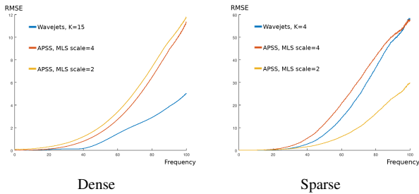
Figure 11: Root Mean Square Error (RMSE) of estimated mean curvature with Wavejets and APSS [GGG08] on the shape of Figure 10. The left chart shows the RMSE computed on the part of the shape where the number of neighbors is strictly greater than 150 so K = 15 . The right chart shows the RMSE computed where the number of neighbors is between 17 and 31. Wavejets of order 4 are computed in such cases. R_\phi is 2.5% of the diameter of the shape.
