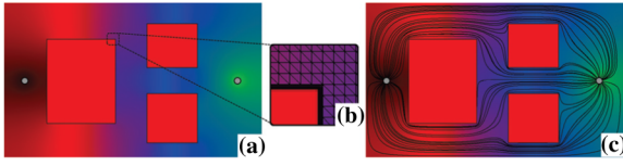
Figure 2: (a) An example of the harmonic field generated for a scene, (b) zoomed-in view showing the right-angled triangles sampled in the space and (c) the guide lines computed over that harmonic field. The value of the harmonic field varies from 0 to 1, which is visualized by the varying colour from red to green.
